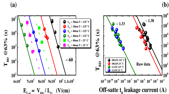
Figure 21. Lifetime plots as T_{BD} at 63% for 28nm N-FET (a) vs. electrical field E_{\max} \cong V_{DS}/L_G enlightening L_G dependence between 25°C (dash lines) and 125°C (solid lines) and (b) vs. drain and gate oxide initial leakage current overcoming L_G dependence between 25°C and 125°C. This shows better lifetime monitoring using gate leakage and slightly more dispersion on drain side in 28nm N-FETs.
