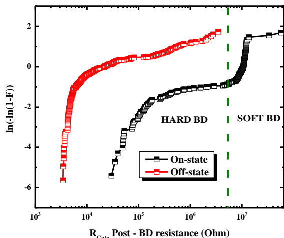
Figure 13. R_{GATE} distribution plot for Off-mode and On-mode TDDB showing multi-modal behaviors between hard BD and soft BD.
