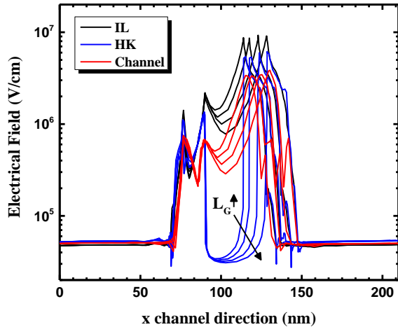
Figure 23. Lateral profile of electrical field during Off-state TDDB in channel, interface layer and high-K for different gate channel length L_G (30nm, 34nm, 40nm, 46nm). Average electrical field is higher for shorter device although the peak value at drain edge is approximately the same for all devices.
