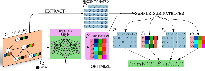
Fig. 1. Architecture of the GRIOT Framework. Given a graph \mathcal{G} = (\mathcal{V}, \mathcal{E}) with nodes attributes F , and a mask of missing data \Omega as input , GRIOT decomposes in 2 main elements : the GCN Imputer and the MultiW Loss Function used to optimize it. The framework outputs the last imputed attributes matrix \hat{F} and the GNN imputer trained and ready to be reused on new nodes with missing attributes.
