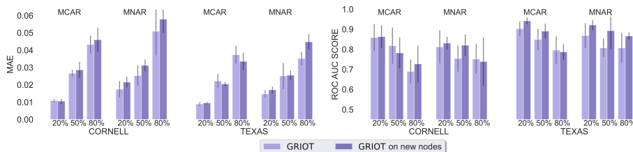
Fig. 3. Performance in terms of (left) MAE and (right) AUC score of GRIOT and GRIOT tested on nodes not present at training time for all settings.
