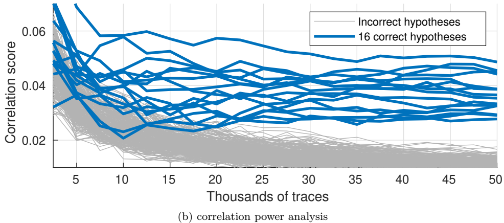
Figure 5: Power analysis of an unprotected implementation of AES running at 100 MHz, sampled at 200 MHz
