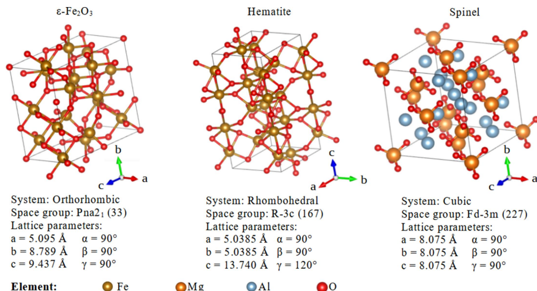
Figure 1 Structures and crystallographic data of \epsilon - \text{Fe}_2\text{O}_3 (ICSD-51122), hematite (ICDD-01-071-5088) and spinel (COD-1540775).
