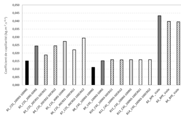
Figure 7. Coefficient de capillarité
