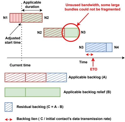
Fig. 3. The bundle depicted by the blue diagonally striped box cannot be fragmented; therefore, the second contact is not fully utilized. The applicable backlog does not cover a portion of its applicable prior volume. This volume portion would still be subtracted from the applicable backlog to calculate the residual backlog needed for ETO calculation.
