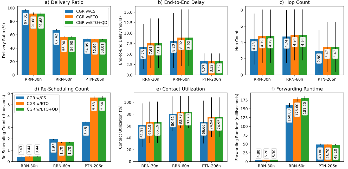
Fig. 8. Evaluation results across three scenarios (RRN-30n, RRN-60n, and PTN-206n) using three volume management techniques (CS, ETO, and ETO+QD). The top figures (a, b, and c) present the benefits in terms of delivery ratio, delay, and path length, respectively. The figures on the bottom (d, e, f) illustrate the costs of achieving the benefits: re-forwarding effort, contact utilization, and computational costs, respectively. In all cases, the bar plots present the averaged values across all nodes in the 20 simulations (bars include the average numerical annotation), and the error bars illustrate the standard deviation.
