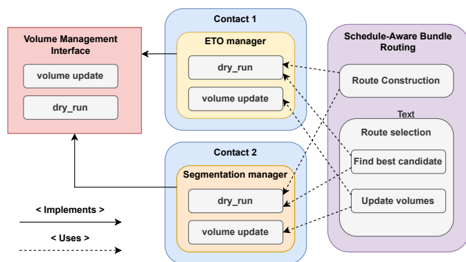
Fig. 7. Interactions between the proposed Volume Management Interface, the volume manager implementations, and SABR specification architecture.
