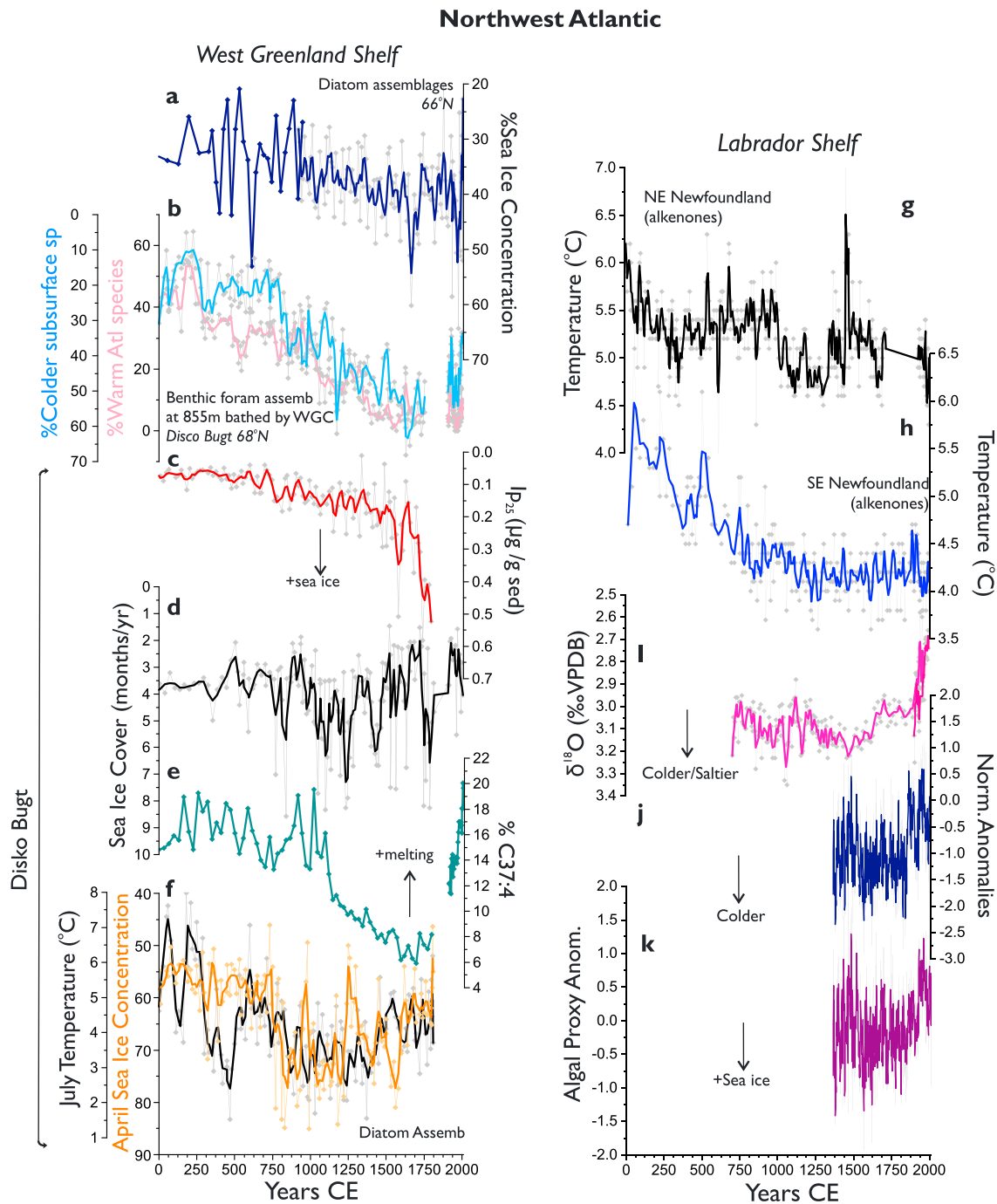
Figure 6. Ocean conditions around West Greenland and the Labrador Shelf. (a) Sea ice concentration from central west Greenland shelf (GA306-BC/GC4 spliced with lower res GA306-GC3; Sha et al., 2016; Sha et al., 2017), (b) benthic foraminifera assemblages at 855 m on the West Greenland Shelf bathed by WGC (343310-MC/GC; Perner et al., 2011), Disco Bugt surface ocean reconstructions; (c) biomarker sea ice reconstructions (343310GC; Kolling et al., 2018); (d) sea ice cover reconstructed from dinocysts (343310-MC/GC; Allan et al., 2018); (e) organic biomarkers as indicators of melting (343310; Moros et al., 2016), (f) diatom assemblages July sea surface temperature reconstructions (black) and April sea ice cover (343310; (Krawczyk et al., 2017); (g) alkenone-based sea surface temperatures from NE Newfoundland (AI07-04BC/3G) and (h) (AI07-11BC/12G; Sicre et al., 2014). (i) Benthic \delta^{18}\text{O}_{\text{foram}} record at 300 m within the Laurentian Channel GR02-23 and MD99-2220 (Thibodeau et al., 2018). (j) Multispecimen record of coralline algae from Labrador and Baffin Island generated by averaging the normalized and annually averaged Mg/Ca (Moore et al., 2017) and (k) annual growth rates (Halfar et al., 2013) giving equal weight to each of the time series. Bold lines on raw data are weighted three-point smoothing.
