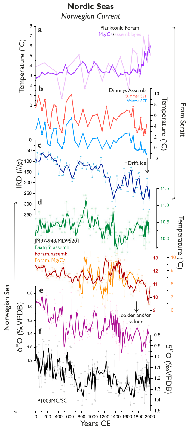
Figure 4. Properties of Atlantic Inflow waters in the Nordic Seas. Fram Strait (a) MSM05/5_712-1: Planktonic foraminifera assemblages and Mg/Ca temperature indicators (Spielhagen et al., 2011); (b) JM06-WP-04-MCB: Dinocyst assemblages (Bonnet et al., 2010); (c) ice-rafted debris counts per gram (MSM5/5-712-1; Werner, Spielhagen, et al., 2011); Voring Plateau core JM97-948/MD952011 surface ocean reconstructions; (d) temperatures based on diatom assemblages (green; Berner et al., 2011), Mg/Ca composition of planktonic foraminifera (orange; Nyland et al., 2006) and planktonic foraminifera assemblages (burgundy; Andersson et al., 2003); (e) \delta^{18}\text{O}_{\text{foram}} (Risebrobakken et al., 2003); and (f) \delta^{18}\text{O}_{\text{foram}} from P1003MC/SC (Sejrup et al., 2011). Bold lines on raw data are weighted three-point smoothing.
