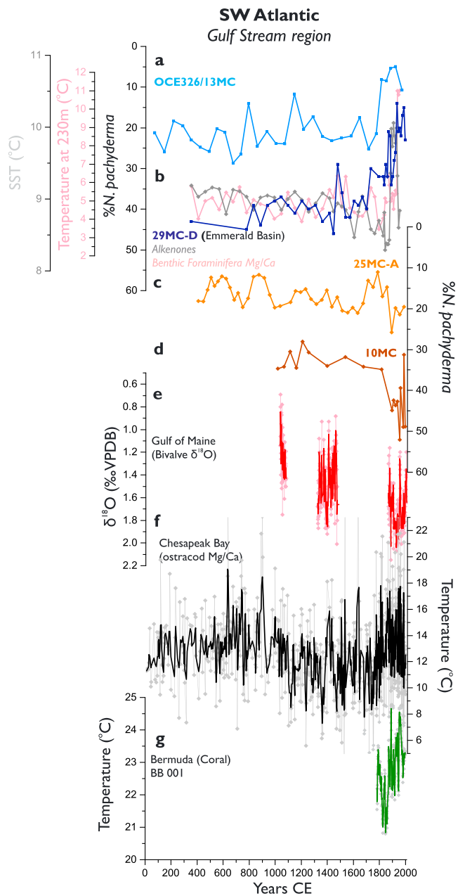
Figure 2. Surface ocean records from the southwest and northwest Atlantic. Percentages of the polar foraminiferal species N. pachyderma from (a) Laurentian Fan (Keigwin & Pickart, 1999) (b) Nova Scotia (Emerald Basin; blue; note that superimposed are two records from the same core: Mg/Ca-based temperatures based on benthic foraminifera C. lobatus , in pink, and sea surface temperature (SST) record from alkenones, in gray (Keigwin et al., 2003); (c, d) % N. pachyderma from Laurentian Fan (25MC-A and 10MC, respectively; Thornalley et al., 2018); (e) \delta^{18}\text{O} from the bivalve Arctica islandica from the Gulf of Maine (Wanamaker et al., 2008); (f) Ostracod Mg/Ca-based temperature reconstructions based on three spliced sediment cores from Chesapeake Bay (Cronin et al., 2010); (g) temperature reconstructions based on Sr/Ca in brain coral from Bermuda (Goodkin et al., 2008). Bold lines are weighted three-point smoothing.
