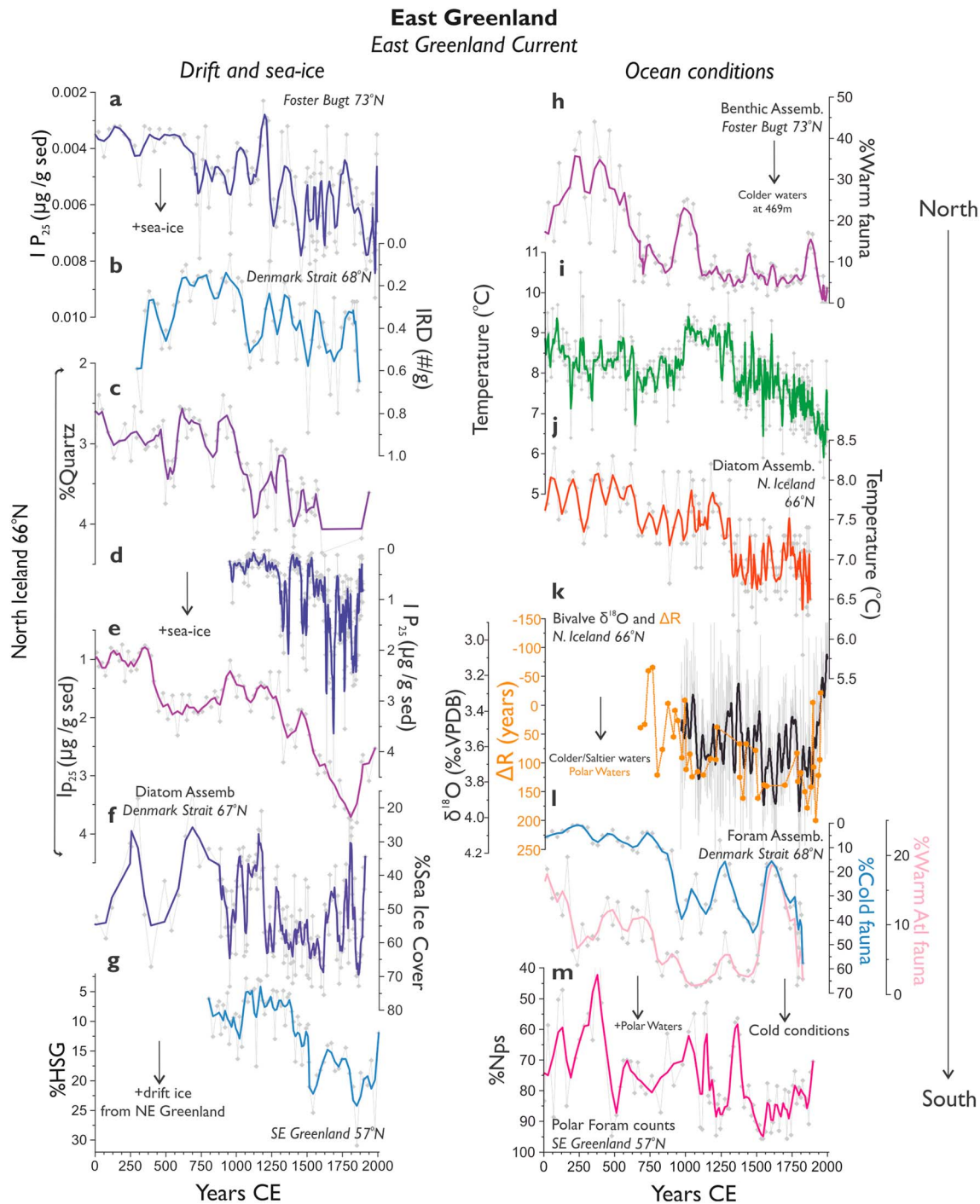
Figure 5. Ice and oceanographic conditions along Eastern Greenland and North Iceland. Left panel shows sea/drift ice conditions (a) sea ice conditions in PS2641 BC/GC at Foster Bugt (Kolling et al., 2017); (b) drift ice recorded in the Denmark Strait JM96-1206/2GC (Perner et al., 2016) North Iceland; (c) %Quartz from MD99-2269 (Moros et al., 2006); sea ice biomarker (d) MD99-2275 (Massé et al., 2008) and (e) MD99-2269 (Cabedo-Sanz et al., 2016); (f) April sea ice cover from diatom assemblages in the West Denmark Strait (MD99-2322; Miettinen et al., 2015); and (g) Haematite Stained Grains (HSG) transported from northwest Greenland to South Greenland (GS06-144-03; Alonso-Garcia et al., 2017). Right panel shows oceanographic conditions (h) benthic foraminiferal assemblages at ~430 m, which are indicator of Atlantic Intermediate Waters (PS2641 BC/GC; Perner et al., 2015), North Iceland upper water column conditions; (i) sea surface temperatures from alkenones (MD99-2275; Sicre et al., 2008; Sicre et al., 2011); (j) summer sea surface temperatures from diatom assemblages (Jiang et al., 2015; MD99-2275); (k) \delta^{18}\text{O}_{\text{shell}} (black; Reynolds et al., 2016) and \Delta R (orange; Wanamaker et al., 2012) from Arctica islandica from the North Iceland shelf; (l) benthic assemblage from ~400-m deep in the Northern Denmark Strait (JM96-1206/2GC; Perner et al., 2016); (m) % planktonic foraminifera species N. pachyderma from the Eastern Labrador Sea (South Greenland; RAPiD-35-COM; Moffa-Sánchez & Hall, 2017). Bold lines on raw data are weighted three-point smoothing.
