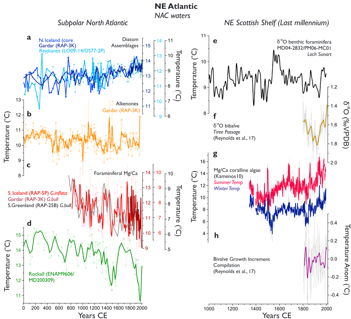
Figure 3. NE Subpolar Atlantic surface reconstructions lying in NAC waters. Left panel: upper water column reconstructions in the Subpolar North Atlantic. Diatom reconstructions from (a) North Iceland MD99-2269 (Justwan et al., 2008), Gardar Drift (RAPiD-21-3K; Miettinen et al., 2012), Reykjanes Ridge LO09-14/DS77-2P (Berner et al., 2008); (b) alkenone records from RAPiD-21-3K (Sicre et al., 2011); foraminiferal Mg/Ca-based temperature reconstructions from (c) RAPiD-17-5P south of Iceland based on the near-thermocline dweller G. inflata (Moffa-Sanchez et al., 2014), and the 230-year record from the surface dweller G. bulloides RAPiD-21-12B Gardar Drift (Hall et al., 2010), RAPiD-35-25B (same location as RAPiD-35-COM, Figure 1) South Greenland (Moffa-Sanchez et al., 2014); and (d) Rockall Trough ENAM9606/MD2003209 (Richter et al., 2009). Right panel: upper water column temperature reconstructions from the Scottish Shelf (e) Loch Sunart temperature calculated based on the \delta^{18}\text{O}_{\text{foram}} assuming no salinity changes (Cage & Austin, 2010), (f) Tiree Passage \delta^{18}\text{O}_{\text{shell}} (Reynolds et al., 2017), (g) Coralline algae Mg/Ca-based winter and summer temperatures (Kamenos, 2010), and (h) proxy network temperature anomalies with respect to the series mean based on bivalve growth increments (Reynolds et al., 2017). Bold lines on raw data are weighted three-point smoothing.
