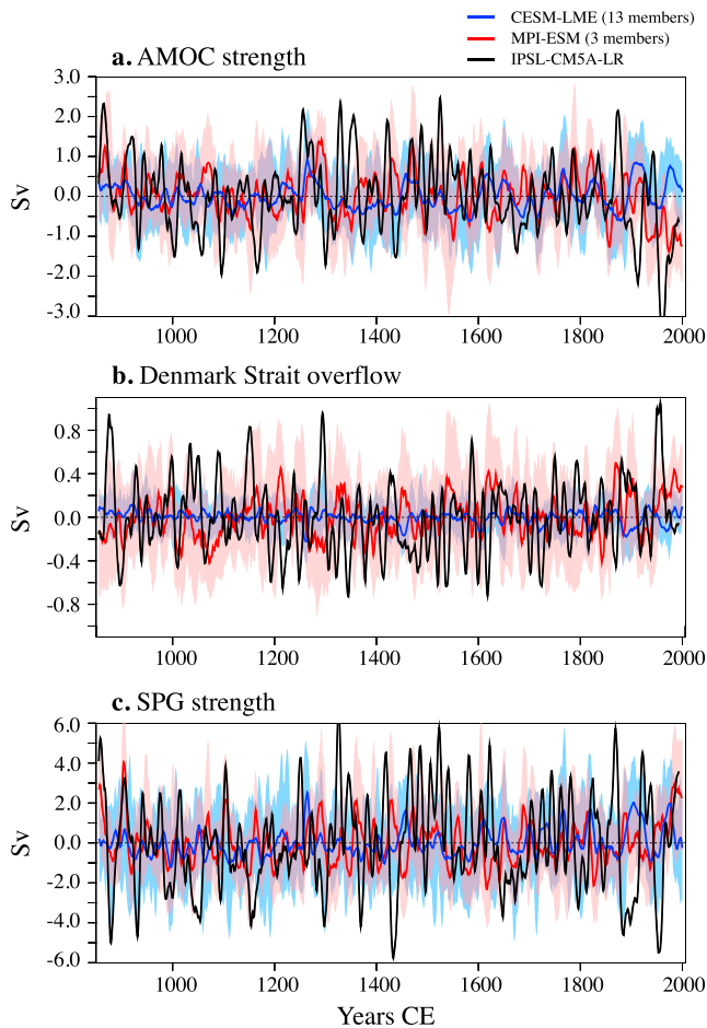
Figure 8. Simulated evolution over the last millennium for the three selected models of three key ocean circulation variables, expressed in Sv ( 1 \text{ Sv} = 10^6 \text{ m}^3/\text{s} ): (a) the AMOC strength (defined as the average of the overturning stream function between 35^\circ\text{N} – 50^\circ\text{N} and 500 – 1,500 \text{ m} ), (b) the Denmark Strait overflow (computed as the southward mass transport of dense waters across the Denmark Scotland Ridge; for the exact definition see section 3.2), and (c) the SPG strength (estimated as the maximum absolute value of the barotropic stream function between 50^\circ\text{N} – 65^\circ\text{N} and 20^\circ\text{W} – 60^\circ\text{W} ). All values are shown as anomalies with respect to the complete simulated period. The red and blue envelopes respectively represent the total MPI and CESM ensemble spreads (i.e., from the minimum to the maximum values across all members).
