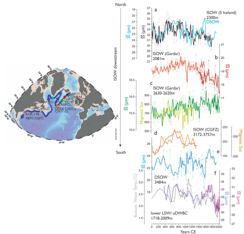
Figure 7. Deep (>1,700 m) ocean records from the subpolar North Atlantic. Inset map outlining the deep circulation boundary currents in the Subpolar North Atlantic including the Nordic Overflows (ISOW and DSW) and the Deep Western Boundary Current (DWBC), with the proxy record locations indicated by circles color coded to the data in the graph. Bathymetric base map is made using Ocean Data View (ODV; (Schlitzer, 2015)). The graph is ordered from the ISOW from north to south including (a) RAPiD-17-5P, which is south of Iceland and close to the Greenland-Scotland Ridge (Moffa-Sanchez et al., 2015; note that the SS from the DSW, also shown in (e) has been plotted in blue in reverse to show the antiphasing); (b) GS06-144-09MC (dark red; (Mjell et al., 2016) and GS06-144-08GC (red; (Mjell et al., 2015; note the discrepancy when splicing); (c) Southern Gardar drift SS from RAPiD-21-3K (Moffa-Sánchez & Hall, 2017) and magnetic susceptibility from MD99-2251 (Kissel et al., 2013); (d) magnetic susceptibility from the deep Charles Gibbs Fracture Zone (CGFZ) CH77-02 and DD08-3182C1 (Kissel et al., 2013); (e) SS record from the from RAPiD-35-COM in the Eirik Drift off the southern tip of Greenland in the path of the DSW (Moffa-Sanchez et al., 2015); and (f) sortable silt record from KNR-178-48JPC/56JPC in the pathway of lower LSW/upper DWBC (uDWBC; Thornalley et al., 2018). The record in grey denotes three-point smoothed benthic foraminiferal Mg/Ca temperatures at 1,845 m on the Scotian Shelf interpreted as deep LSW (Marchitto & de Menocal, 2003; note that the data from the top 23.5 cm of this record were plotted on the updated age model for KNR-158-10MC from Thornalley et al., 2018). Bold lines on raw data are weighted three-point smoothing.
