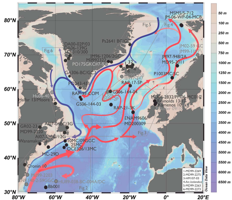
Figure 1. Regional schematic map of the surface ocean currents. Based on Orvik and Niiler (2002), Daniault et al. (2016), and Bosse et al. (2018). Red arrows indicate the pathway of relatively warm and saline waters and blue arrows the pathway of cold southward polar waters. The locations of the proxy records that are plotted in Figures 2–6 and discussed in this section are indicated by the black (plotted and discussed) and gray (only discussed) circles, respectively. The subregions covered in Figures 2–6 are enclosed by the grey dotted lines and labeled accordingly (base bathymetric map made using Ocean Data View; ODV; Schlitzer, 2015).
