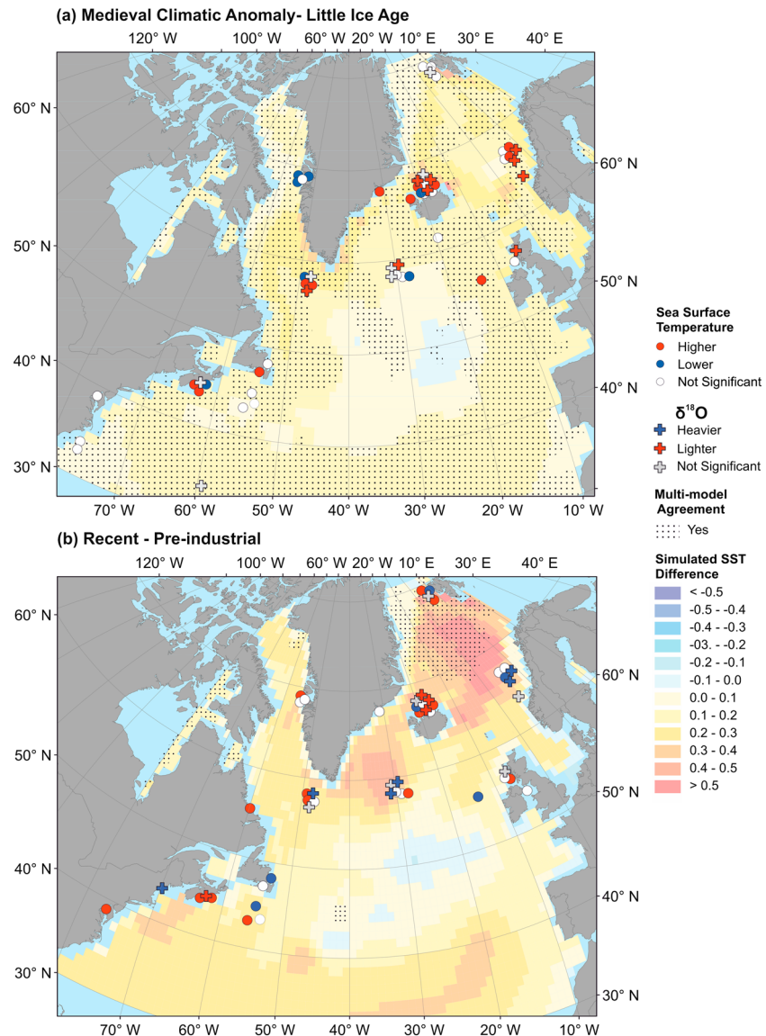
Figure 10. Proxy-model comparison of surface ocean temperature changes in the last millennium. SST (0 m) change simulated by the multimodel ensemble (shaded contours) or reconstructed SST (approximately 0–150 m) by the proxies (filled symbols). Stippling indicates regions in which all models show the same sign of change. In the proxies, colored circles indicate qualitative SST changes between the two periods: red for a warming, blue for a cooling, and white if the change is not significantly different from zero. Colored crosses are equivalent to the circles but represent \delta^{18}\text{O} -based proxies, which are a combination of temperature and salinity. (a) SST differences between the MCA (850–1250 years CE) and the LIA (1450–1850 years CE) (b) SST differences between the industrial (1851–2000 years CE) and the preindustrial (850–1850 years CE) periods (note that for the proxy data 1000–1850 years CE was used for the preindustrial period). See supporting information Table S2 for the details of the data used.
