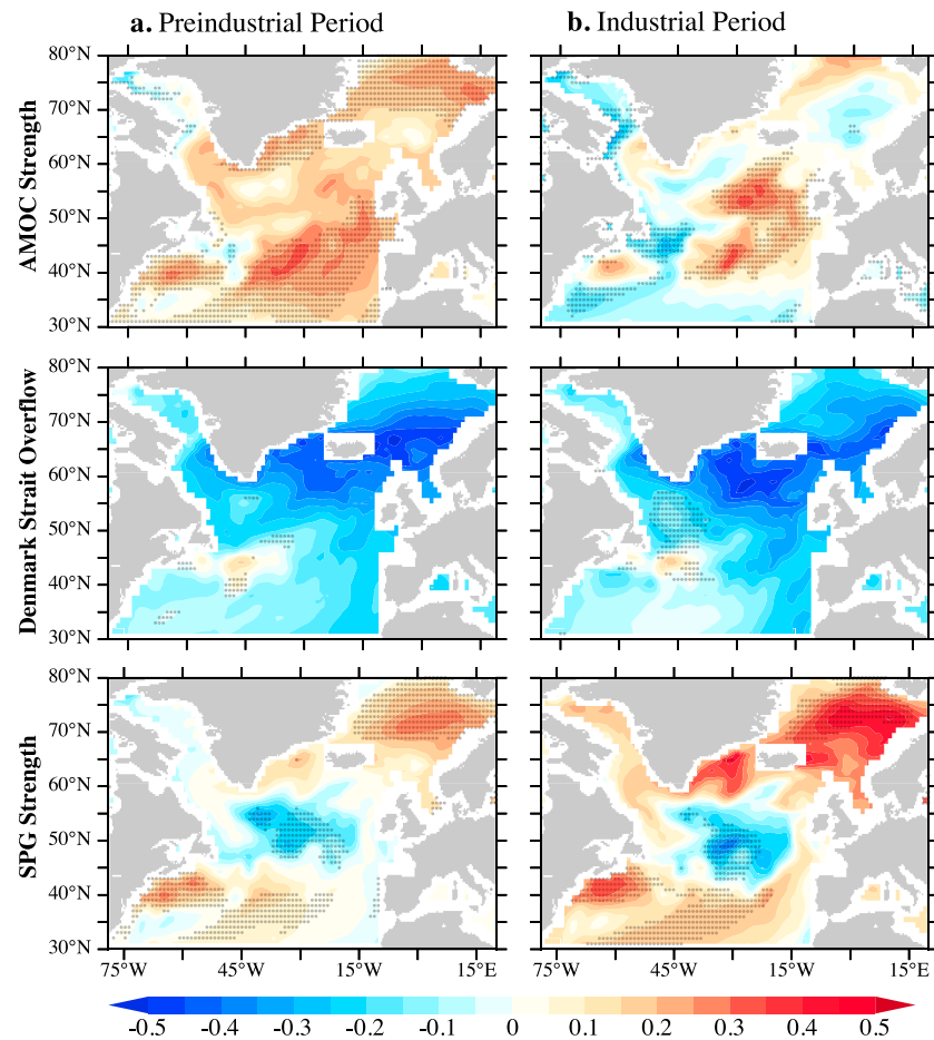
Figure 9. Model SST fingerprints for the ocean circulation and current indices. Regression coefficients (in standard deviation units) between the selected ocean circulation indices (AMOC, DSO, and SPG strength) and the SST fields for the preindustrial (850–1849 CE) and industrial periods (1850–2005 CE). Before regression coefficients are calculated in each individual model simulation, both the SST and the indices are first smoothed with a 10-year running mean and then standardized with respect to each period. The multimodel mean is based on the average of the individual ensemble means of the CESM, the MPI-ESL, and the IPSL-CM5A-LR. Stippling highlights regions of agreement between the three models regarding the sign of the regression coefficient. The ensemble mean of each model is shown in supporting information Figures S1–S3.
