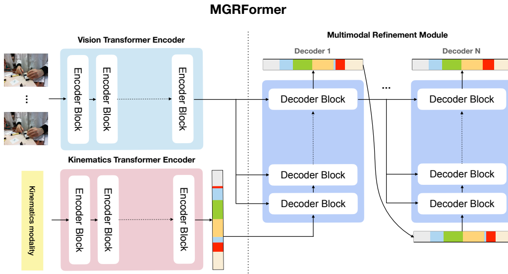
Fig. 1: Illustration of the MGRFormer framework, consisting of two Unimodal Encoders and a Multimodal Refinement Module for iterative cross-refinement using the output predictions of one modality and the Encoder features of the other modality.
