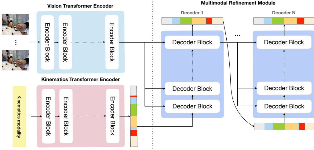
Fig. 1: Illustration of the MGRFormer framework, consisting of two Unimodal Encoders and a Multimodal Refinement Module for iterative cross-refinement using the output predictions of one modality and the Encoder features of the other modality.
