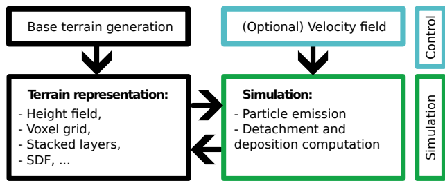
Fig. 5: Our overall pipeline: our erosion process compute matter displacement of a terrain using an arbitrary representation as long as intersections between particles and the ground can be detected. An optional velocity field, provided by the user, guides the particles trajectories. We propose surface alteration methods to apply the erosion to the terrain in a coherent way between possible representations.
