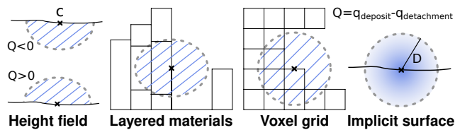
Fig. 6: Illustration of the material detachment in the (half-)sphere at contact point C (cross) on different representations. (height field) When Q < 0 material detachment happen in the bottom scaled half sphere of the particle’s contact with the ground, while the deposition is applied on the upper half sphere of volume when Q > 0 . Unlike the height field, for 3D terrains detachment and deposit are applied in the full sphere around the contact point.
