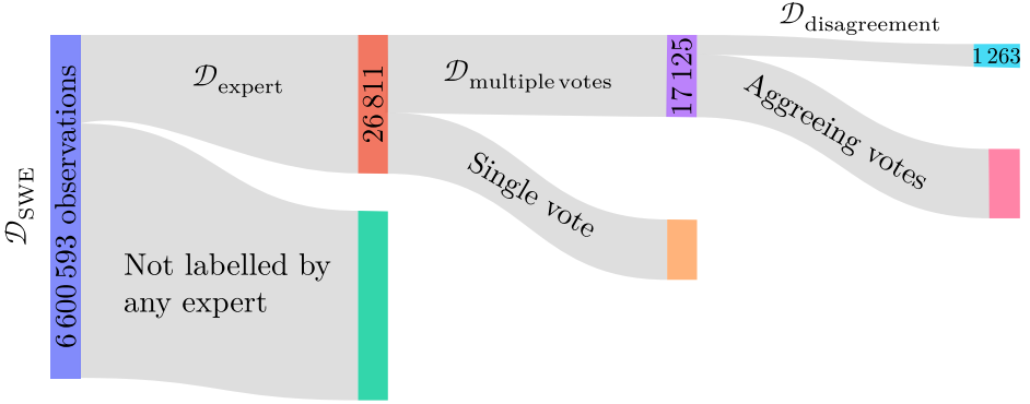
FIG. 3. Log-scales distribution of the observations in the South-West European Flora subset from the PI@ntNet database. Note that the (sub-)datasets introduced are nested: \mathcal{D}_{\text{SWE}} \supset \mathcal{D}_{\text{expert}} \supset \mathcal{D}_{\text{multiple votes}} \supset \mathcal{D}_{\text{disagreement}} . \mathcal{D}_{\text{expert}} and the following subsets contain observations that received at least one vote from one of the experts.
