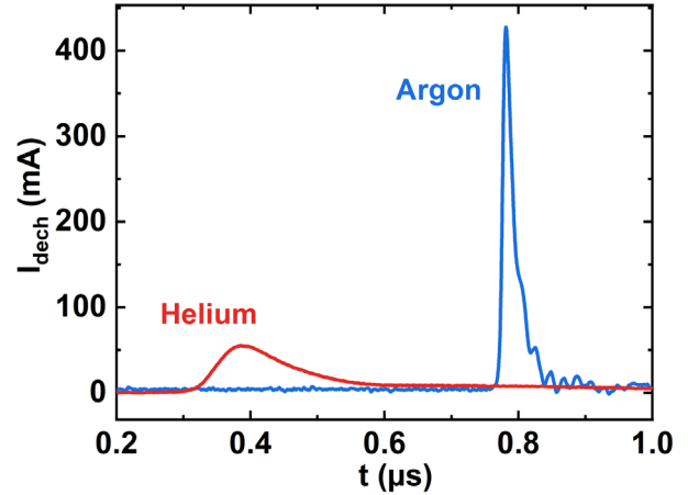
Fig. 10. Temporal representation of the discharge current in Helium/ \text{CO}_2 ( \{99.7/0.3\} %) or Argon/ \text{CO}_2 ( \{99.7/0.3\} %). The data were recorded at 20 kHz with a total gas flow rate of 1000 sccm and a frequency of 20 kHz.
