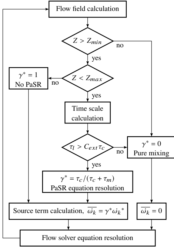
Figure 5 Flowchart for the flow solution calculation procedure using the PaSR model and the extinction model (adapted from Sloan and Sturgess [16]).
