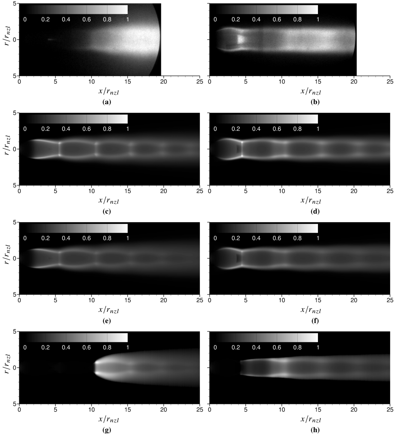
Figure 10 Comparison of the normalized level of mean \text{OH}^* chemiluminescence emission measured by the UV camera with the simulated normalized level of Abel transform of mean heat release \omega_T in (left) the static case and (right) the dynamic case; (10a and 10b) camera measurements; (10c and 10d) simulations under QL approximation; (10e and 10f) simulations with PaSR model alone; (10g and 10h) simulations with PaSR and extinction models.
