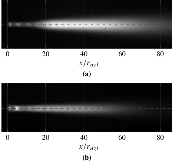
Figure 3 Mean contrast radiance field in grayscale obtained from the NOXANT infrared camera measurements in (3a) the static case and (3b) the dynamic case.
