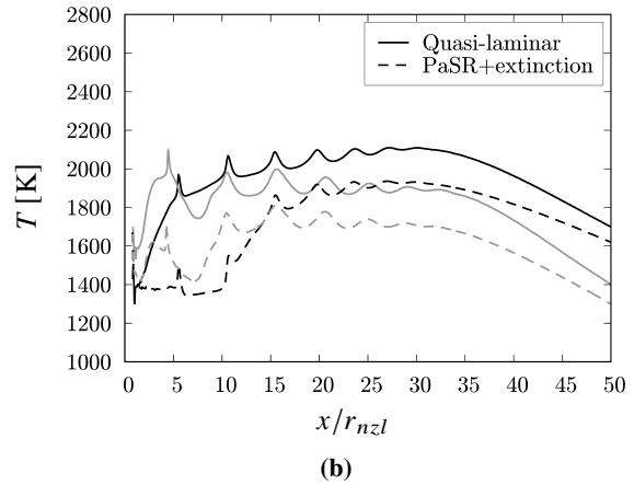
Figure 13 Simulated temperature profiles along (13a) the jet axis and (13b) the line define at the radial location of maximum k inside the mixing layer; black lines: static case; grey lines: dynamic case.
