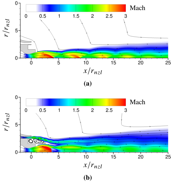
Figure 8 Simulated Mach number fields and streamlines in (8a) the static case and (8b) the dynamic case.
