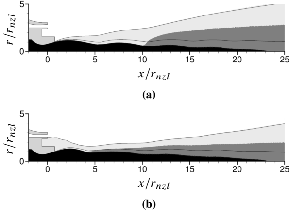
Figure 12 Isolines of Z \in [Z_{min}, 0.5, Z_{max}] superimposed on the contour plot of the extinction model switch regions, in (12a) the static case and (12b) the dynamic case; black region: Z > Z_{max} and \gamma^* = 1 ; dark grey region: PaSR resolution; light grey region: extinction and \gamma^* = 0 ; white region: Z < Z_{min} and \gamma^* = 0 .
