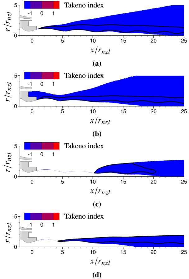
Figure 11 Isolines of heat release \omega_T = 0.1\omega_{Tmax} superimposed on the Takeno index inside the reactive ( \omega_T > 0 ) mixing layer; simulations under QL approximation in (11a) the static case and (11b) the dynamic case; simulations with PaSR and extinction models in (11c) the static case and (11d) the dynamic case.
