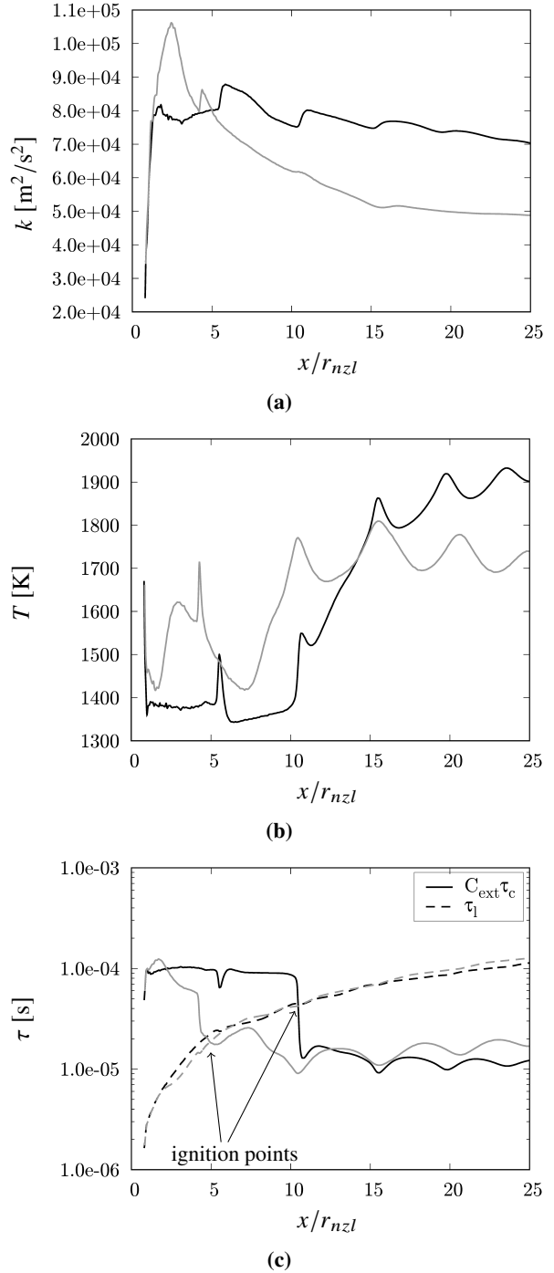
Figure 9 Simulated profiles of (9b) temperature T , (9a) turbulent kinetic energy k and (9c) extinction time scale C_{ext}\tau_c and turbulent time scale \tau_t , along the line define at the radial location of maximum k inside the mixing layer; black lines: static case; grey lines: dynamic case.
