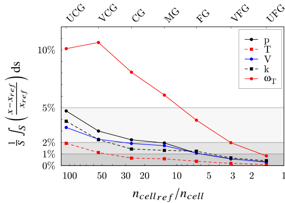
Figure 7 Grid convergence study; mean relative error on pressure, temperature, velocity, turbulent kinetic energy and heat release, along the Z = 0.5 isoline of curvilinear abscissa s .
