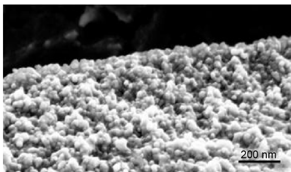
Figure 4 Field emission scanning electron micrograph showing the granular structure of the oxide layer at nanoscale.
