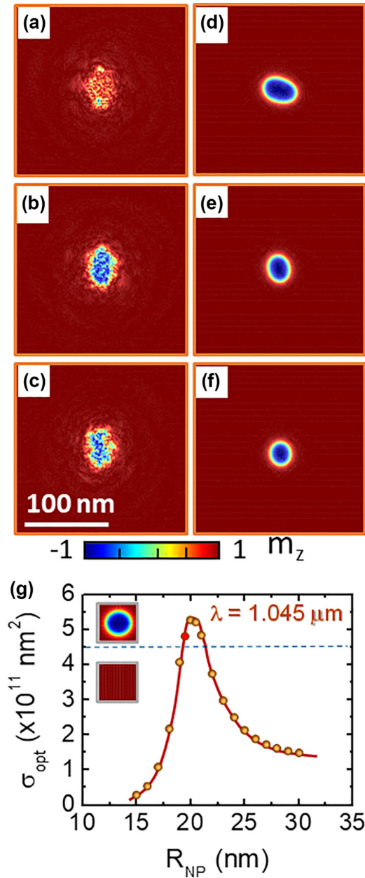
FIG. 3. (a)–(d) Evolution of the skyrmion formation at (a) 100 ps, (b) 200 ps, (c) 300 ps, (d) 500 ps, (e) 700 ps, and (f) 900 ps. (g) Optimal at wavelength of 1045 nm for different gold nanoparticle sizes. The color scale denotes the z component of the spins.
