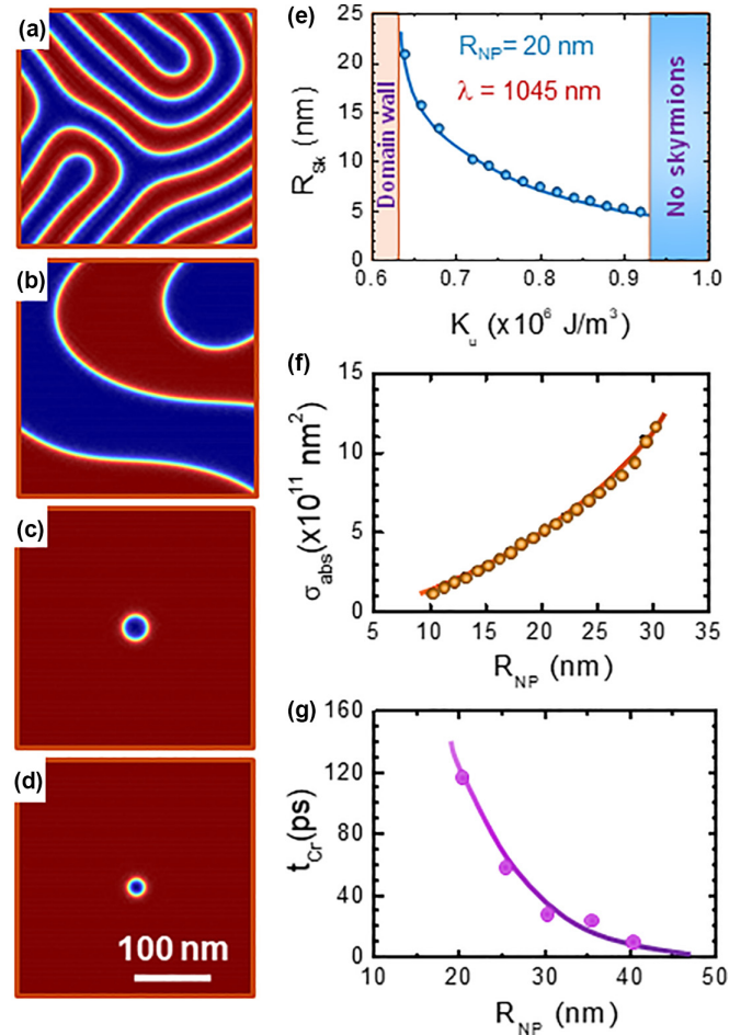
FIG. 4. (a)–(d) Snapshots of magnetization profile showing plasmonic effect on a 20-nm-radius gold nanoparticle for K_u of 0.55, 0.60, 0.65, and 0.70 MJ/m 3 , respectively. (e) Relationship between skyrmion radius and uniaxial anisotropy constant. (f) Absorption cross section as a function of gold NP radius. (g) Creation time of skyrmion versus gold NP radius.
