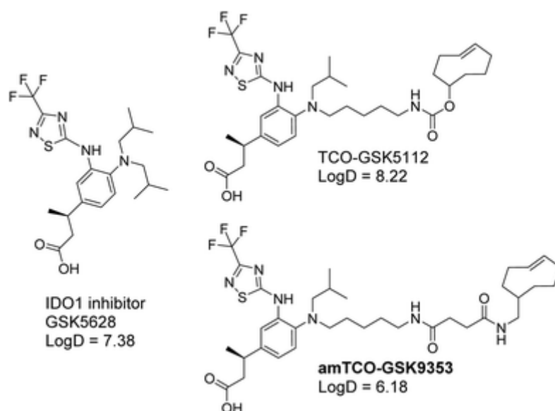
Fig. 3 Structure and log D value of the parent compound GSK5628 and derived click probes.
