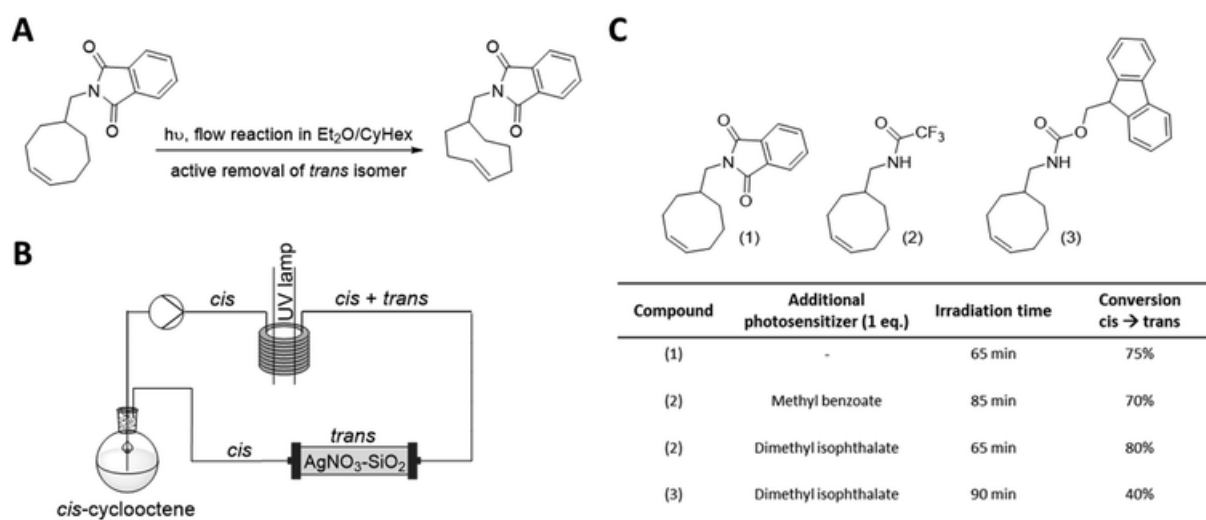
Fig. 2 (A) Photoisomerization of amCCO into amTCO using a phthalimide protecting group as intramolecular photosensitizer. (B) Photoisomerization setup for irradiation of cis -cyclooctenes at 254 nm in continuous flow with trapping of trans -cyclooctenes on silver nitrate-coated silica. (C) Comparative study of different photoisomerization conditions.
