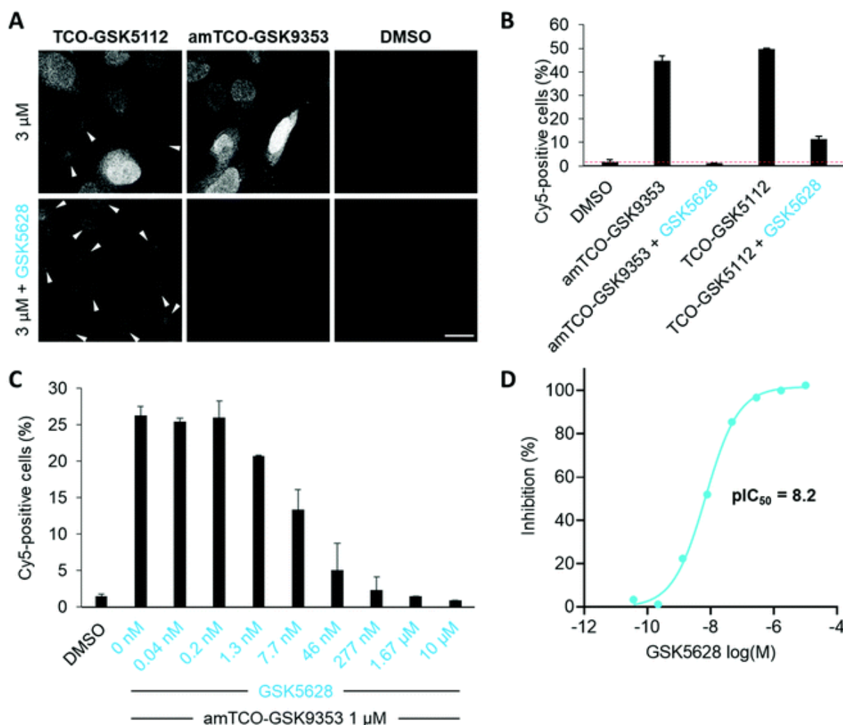
Fig. 4 (A) Imaging assay. IFN \gamma -treated HeLa cells were incubated with 3 \mu M click probe \pm GSK5628 for 1 h, followed by fixation, permeabilization and click reaction with 200 nM Cy5-Tetrazine. Representative fluorescent images recorded after excitation at 633 nm (Cy5, \lambda_{em} = 638–690 nm) are shown. Scale bar = 20 \mu m. The white arrows point at the unspecific accumulation of TCO-GSK5112. (B) Quantification of Cy5 fluorescence signal in HeLa cells treated as in A and analysed by flow cytometry. Dashed line shows DMSO level. Data from one representative experiment (replicates shown in Fig. S27, ESI \dagger ). (C) Flow cytometric analysis of IFN \gamma -induced HeLa cells treated with 1 \mu M amTCO-GSK9353 and increasing concentrations of GSK5628, followed by trypsinization, fixation, permeabilization and click reaction with Cy5-Tetrazine. Data from one representative experiment (replicates shown in Fig. S29, ESI \dagger ). (D) Competition binding curve of GSK5628 derived from flow cytometric data presented in C.
