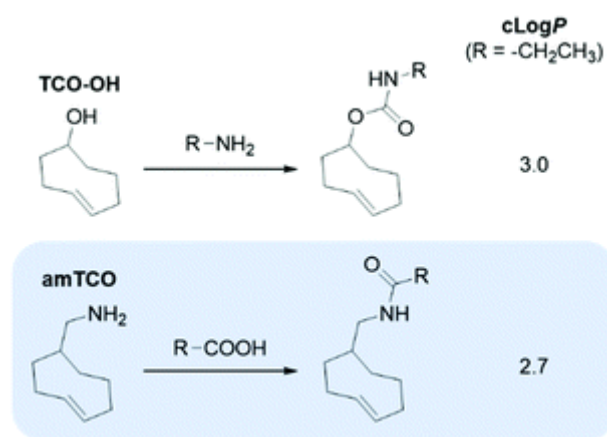
Fig. 1 Structures of TCO-OH and amTCO, and calculated log P values (clog P ) for TCO-OH and amTCO conjugates.
