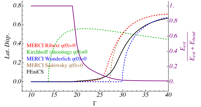
Fig. 31. Lateral Torsional Buckling bifurcation curve with \nu = 0.35 , \frac{w}{L} = 0.4 , and \frac{h}{L} = 0.001 . Note that in the MERC1 code the constraints \eta(0) = 0 and |w\eta'| \leq 2 have been applied.
