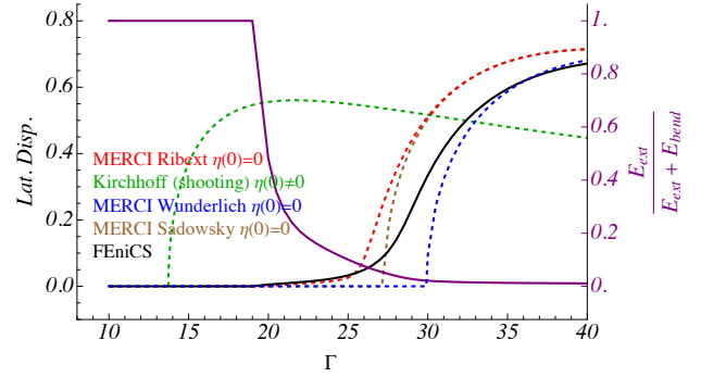
Fig. 31. Lateral Torsional Buckling bifurcation curve with \nu = 0.35 , \frac{w}{L} = 0.4 , and \frac{h}{L} = 0.001 . Note that in the MERC1 code the constraints \eta(0) = 0 and |w\eta'| \leq 2 have been applied.
