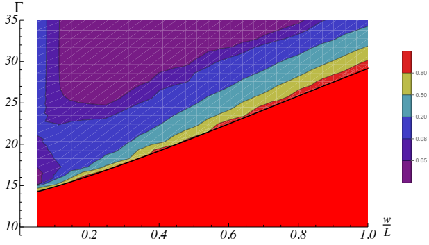
Fig. 21. Contour plot of the energy ratio E_{ext}/(E_{ext} + E_{bend}) computed with the FENICS-SHELL code. Before buckling (under the black curve), only stretching is present. After buckling (above the black curve) there are large parts of the diagram where the extension energy is at least 5% of the total deformation energy.
