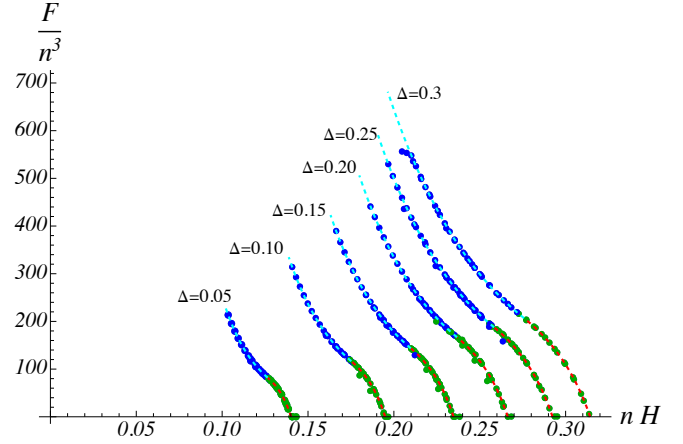
Fig. 24. Vertical force F on the cell with the scaling for both axes as introduced by Roman and Pocheau [1999]. Dotted lines correspond to analytical solutions of the planar Elastica with lineic and planar contact, and points correspond to numerical MERCI data.
