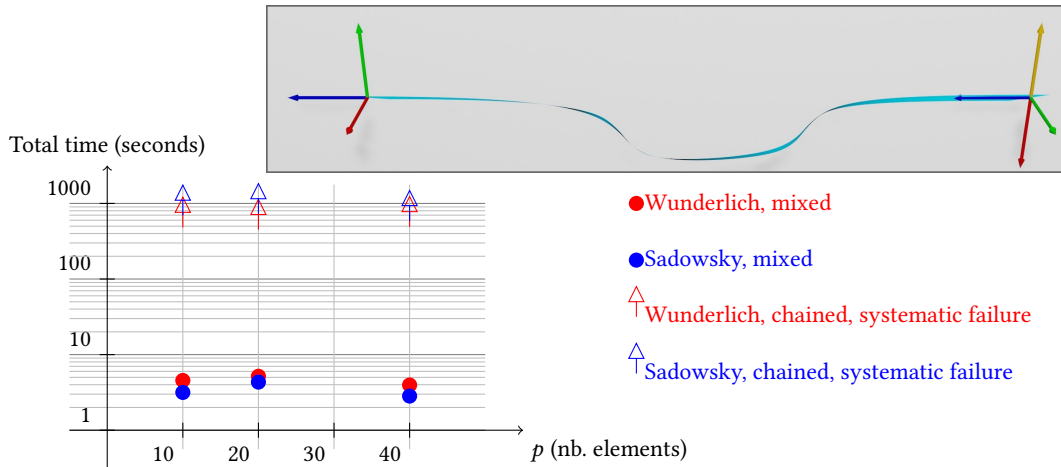
Fig. 6. Efficiency of the chained and mixed models in the Clamped-clamped Scenario of Section 5.6. The chained model always fails with status «Restoration failed» for Wunderlich energy, or reaches the maximum number of iterations (1000) for Sadowsky energy. This demonstrates the usefulness of the mixed model, which converges within a few seconds. Inset figure: yellow arrow indicates vertical direction, while the red, green, blue arrows indicate the orientations at the clamps, showing that one quarter of a turn of end-rotation has been applied on the left clamp.
