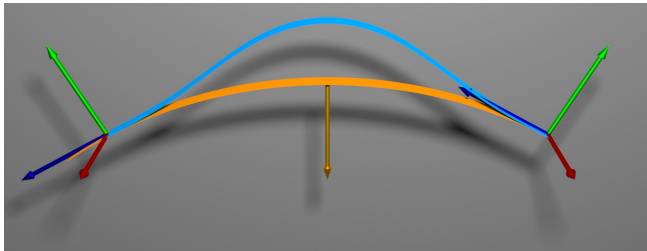
Fig. 4. A simple clamped-clamped experiment. The orange ribbon describes a perfectly circular arc and serves as a warmstart for the minimisation algorithm. This warmstart shape is clamped at the right end, but not at the left end. The two frames are indicating the clamping constraints, and the orange arrow indicates the gravity direction. The blue ribbon is the result of the constrained minimisation. For this experiment, we have used \frac{w}{L} = \frac{1}{11} , \Gamma = 100 , \nu = 0.35 .
