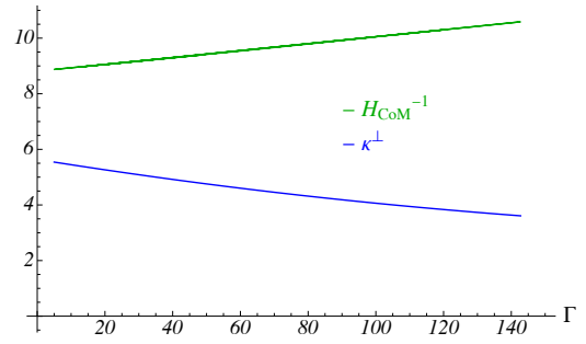
Fig. 15. Is the Möbius ribbon going to roll? Comparison between the distance of the center of mass from the plane, H_{\text{CoM}} , and the curvature \kappa^\perp of the ribbon surface in the direction perpendicular to the ruling at the contact point with the support. ( \frac{w}{L} = 0.025 )
