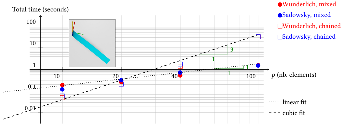
Fig. 5. Efficiency of the mixed and chained models in the Clamped-free scenario of Section 5.6. Computation times are reported and linear and cubic interpolations are shown. The ribbon is hanged under gravity, with a clamping orientation tilted with regard to the gravity vector (inset figure, yellow arrow indicates vertical direction). The mixed model is more efficient when the number of elements is greater than 20 and follows a linear time cost. The chained model is valuable when no more than 20 elements are used, but its time cost increases rapidly, following a cubic trend.
