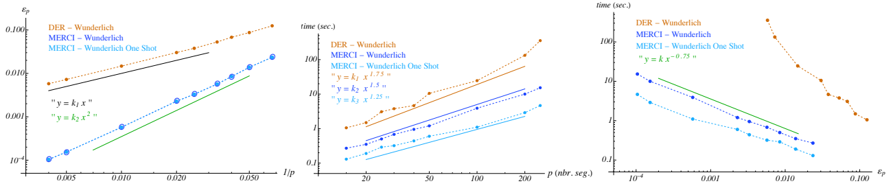
Fig. 12. Comparison between MERCI-WUNDERLICH and DER-WUNDERLICH on the Möbius test, in terms of accuracy and efficiency. Left (log-log scale): Resulting accuracy \varepsilon_p of the Möbius band reached for p elements, function of the length \frac{1}{p} of each element. Middle (log-log scale): Computational time for reaching the Möbius band configuration, function of the number p of elements. Right (log-log scale): Cross-referencing the two left plots, one obtains the computational time required to achieve a given accuracy \varepsilon (regardless of p ), for each tested algorithm.
