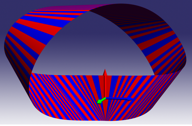
Fig. 7. Möbius solution obtained with MERCY-WUNDERLICH for the normalised width \frac{w}{L} = 0.1 , and the constraints \eta(0) = 0 = \eta(L) . The singular point s = s^* lies at the origin of the cartesian frame. The mesh has been refined so that the increment of the function \eta(s) in any element is not too large, eventually leading to a total number of 169 elements of unequal lengths. The elements are colored alternatively in red and blue, revealing the rulings that lie at the border between two elements.
