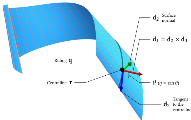
Fig. 3. Kinematics of a developable ribbon.
