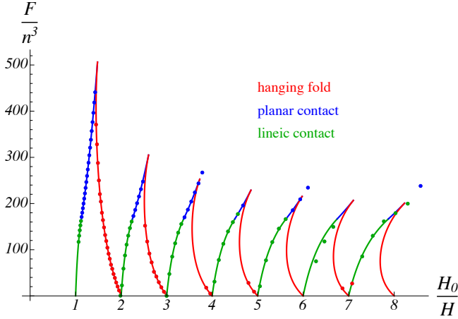
Fig. 19. Total vertical compression force F for \Delta = 0.2 and decreasing height H values. The number n of folds is used to rescale the vertical axis and the height H_0 of the first contact is used to rescale the horizontal axis. The agreement between our semi-analytical solution (solid line) and our numerical results (dots) is excellent.
