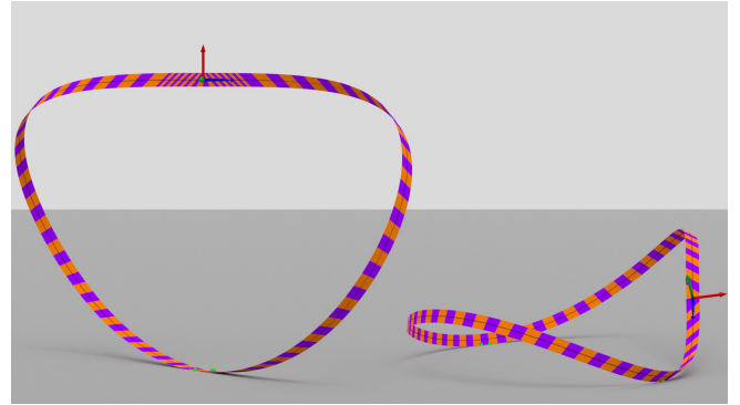
Fig. 13. (Left) the heavy Möbius ribbon stands up on a plane, or (right) the ribbon falls on its side, both solutions being stable. Parameters are \Gamma = 0.1 and \frac{w}{L} = 0.01 .
