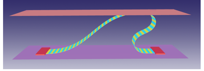
Fig. 18. We retrieve the Spiral configuration recently characterised experimentally by Deboeuf et al. [2024] in the confined ribbon experiment, for \frac{H}{L} = 0.22 and \Delta = 0.4 .
