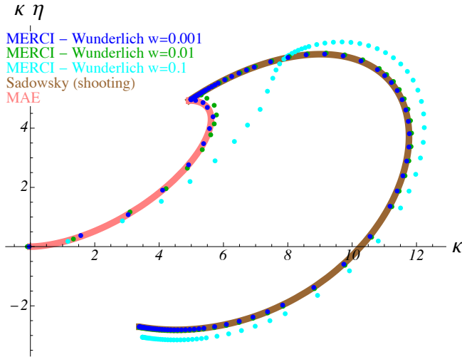
Fig. 8. Parametric plot of the first half of the Möbius solution computed with MERCI-WUNDERLICH for different width values. We also show the SADOWSKY (shooting) solution in brown (MERCI-SADOWSKY giving exactly the same result) and inner layer of MAE in pink, illustrating the convergence of our MERCI-WUNDERLICH code as w \rightarrow 0 .
