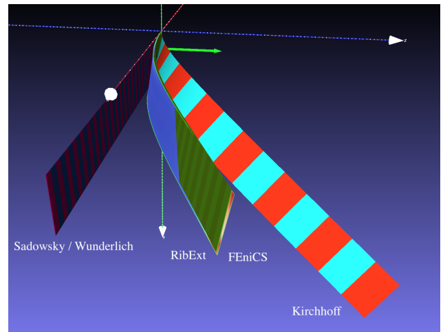
Fig. 23. Equilibrium configurations for the LTB test with \Gamma = 20 , \frac{w}{L} = 0.1 , \frac{h}{L} = 0.001 . While the Sadowsky and Wunderlich models predict an unbuckled shape, the Kirchhoff model predicts a deformation which is too large. Only the RIBEXT model correctly approximates the reference deformation given by the FENICS-SHELL code.
