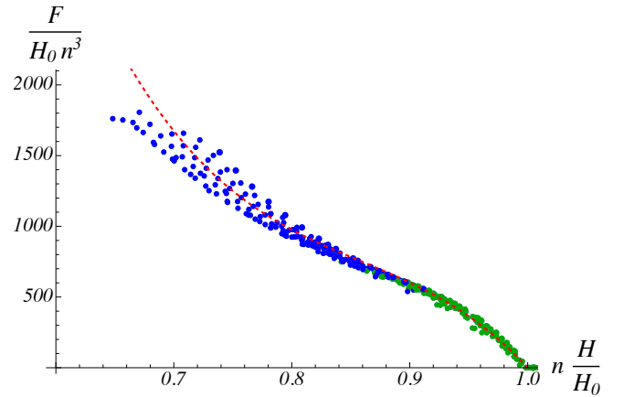
Fig. 25. Approximate collapse of the numerical data of Figure 24 for the vertical compression force F as a function of the height H of the cell, for \Delta = 0.05, 0.1, 0.15, 0.20, 0.25, 0.3 . The number n of waves is such that 1 \leq n \leq 9 , and H_0(\Delta) is the vertical height of the cell at first contact, see Equation (28). The red curve is given by (31).
