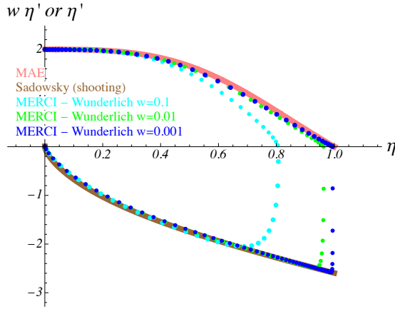
Fig. 30. Parametric plot of the buckled LTB solution with \Gamma = 30 and three values of the width w . Boundary (inner) layer in pink, Sadowsky (outer) solution in brown.
