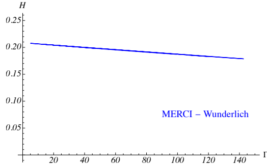
Fig. 14. Height of the Möbius configuration as a function of the weight \Gamma , for \frac{w}{L} = 0.025 .
