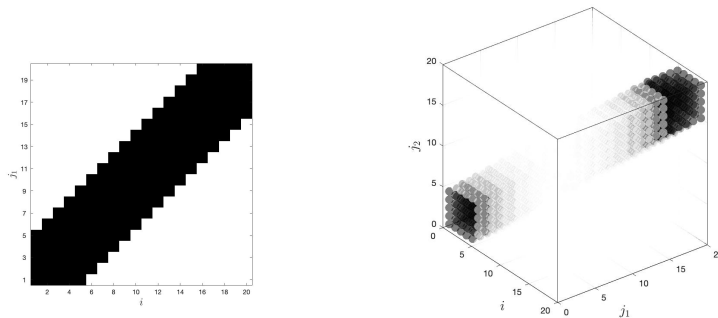
FIGURE 3. Pixel representation of the matrix and 3-tensor respectively corresponding to w^{1, N} and w^{2, N} given by (2.3), with \theta = 0.3 and N = 20 . As this is an unweighted hypergraph, the presence of a hyperedge is represented in black. Transparency was used to indicate depth in the 3-dimensional representation.
