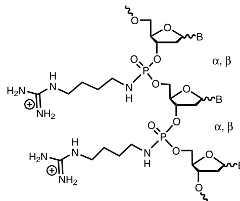
Figure 1. New cationic analogues: guanidinobutylphosphoramidate (PNHBuGua) \beta - or \alpha -oligonucleotides.
