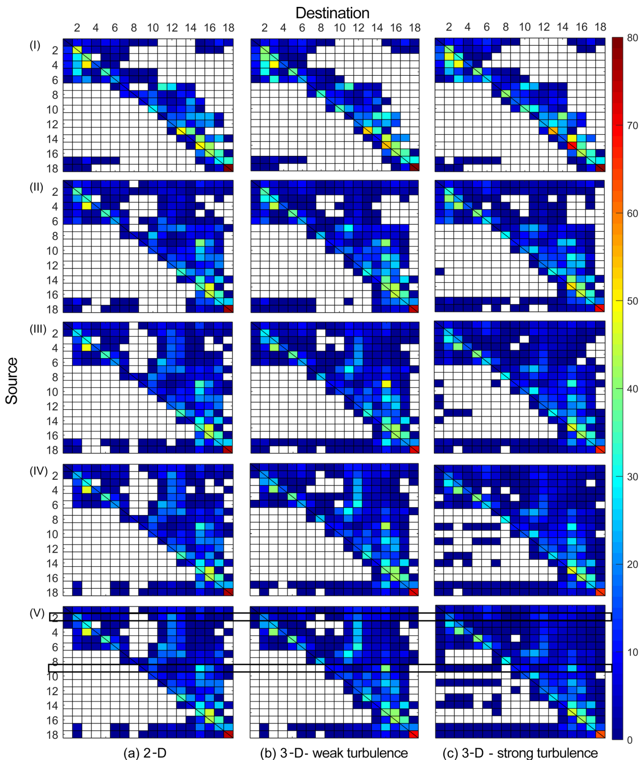
Figure 3. Coastal connectivity between 18 coastal regions in Jervis Bay (Fig. 1) for simulation times (I) 1; (II) 2; (III) 3; (IV) 4; and (V) 5 d, and for the three different scenarios: (a) 2-D approach; (b) 3-D approach with weak vertical turbulence; and (c) 3-D approach with strong vertical turbulence. Each matrix shows the percentage of particles released at source j (vertical axis) that travel to destination i (horizontal axis) for a given simulation time. Black-outlined squares in the lower panels (V) highlight the connectivity for the sources and simulation times in Fig. 2.
