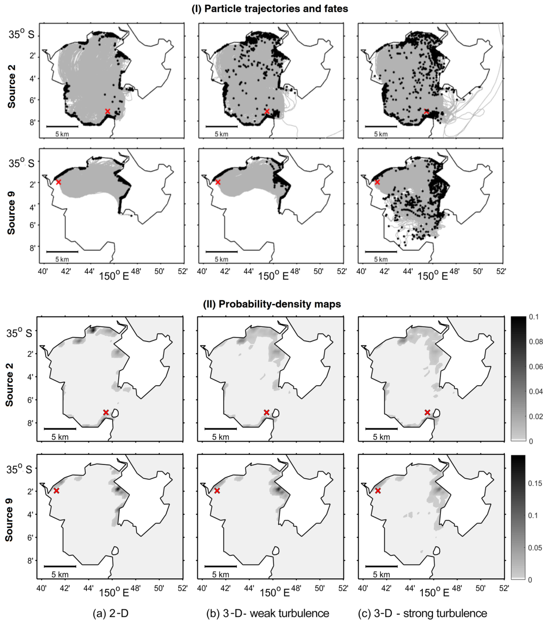
Figure 2. (I) Trajectories (grey lines), fate (black dots) and (II) probability-density distribution (greyscale bar) of microplastics released at sources 2 and 9 (red crosses) after 5 d of simulation for the three different scenarios: (a) 2-D approach; (b) 3-D approach with weak vertical turbulence; (c) 3-D approach with strong vertical turbulence.
