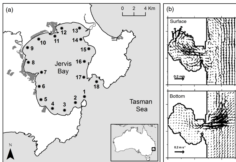
Figure 1. (a) Map of Jervis Bay (south-eastern Australia). Black dots show the seeding locations and also the centre of destination regions used in the coastal connectivity analysis. Shaded areas represent urban zones. (b) Typical surface and bottom currents of the bay (modified from Wang and Symonds, 1999).
