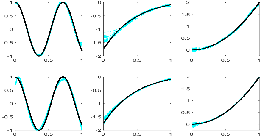
FIGURE 2. Case 1. Estimation of b_1 left, b_2 middle and b_3 right, with basis T (first line) and basis L (second line) for 25 paths. 100 \times \text{MISE}(b_1, b_2, b_3) , (0.284, 0.006, 0.134) for T and (0.748, 0.001, 0.032) for L. Mean of the selected dimensions (5.6, 3.6, 5.5) for T and (6, 0, 2.0, 4.0) for L.
