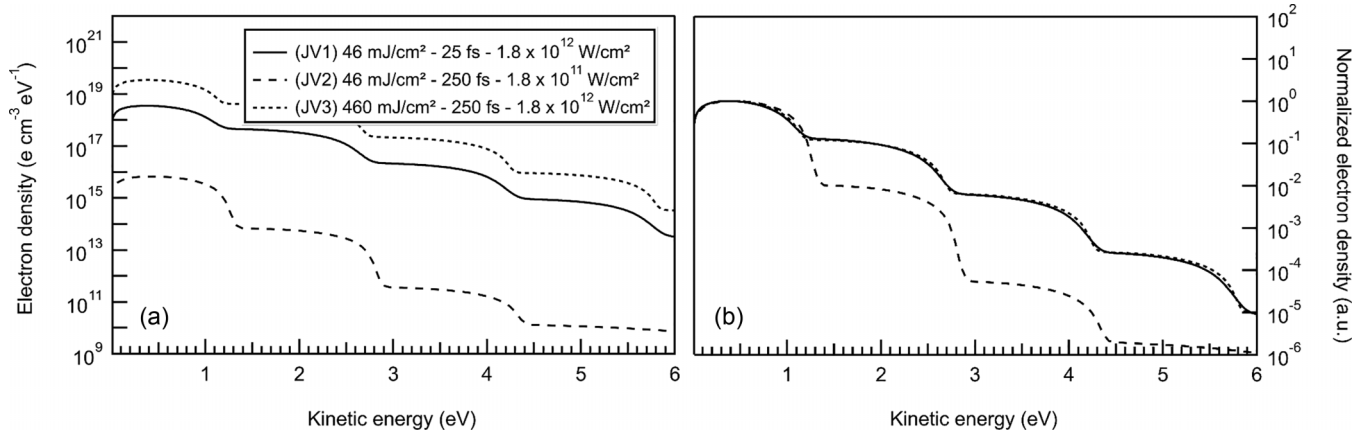
FIG. 5. (a) Initial pump spectrum using the jellium-Volkov approximation for three laser beam configurations: (1) JV1 = 46 \text{ mJ/cm}^2 - 25 \text{ fs} - 1.8 \times 10^{12} \text{ W/cm}^2 ; (2) JV2 = 46 \text{ mJ/cm}^2 - 250 \text{ fs} - 1.8 \times 10^{11} \text{ W/cm}^2 ; (3) JV3 = 460 \text{ mJ/cm}^2 - 250 \text{ fs} - 1.8 \times 10^{12} \text{ W/cm}^2 . (b) Corresponding normalized spectra.
