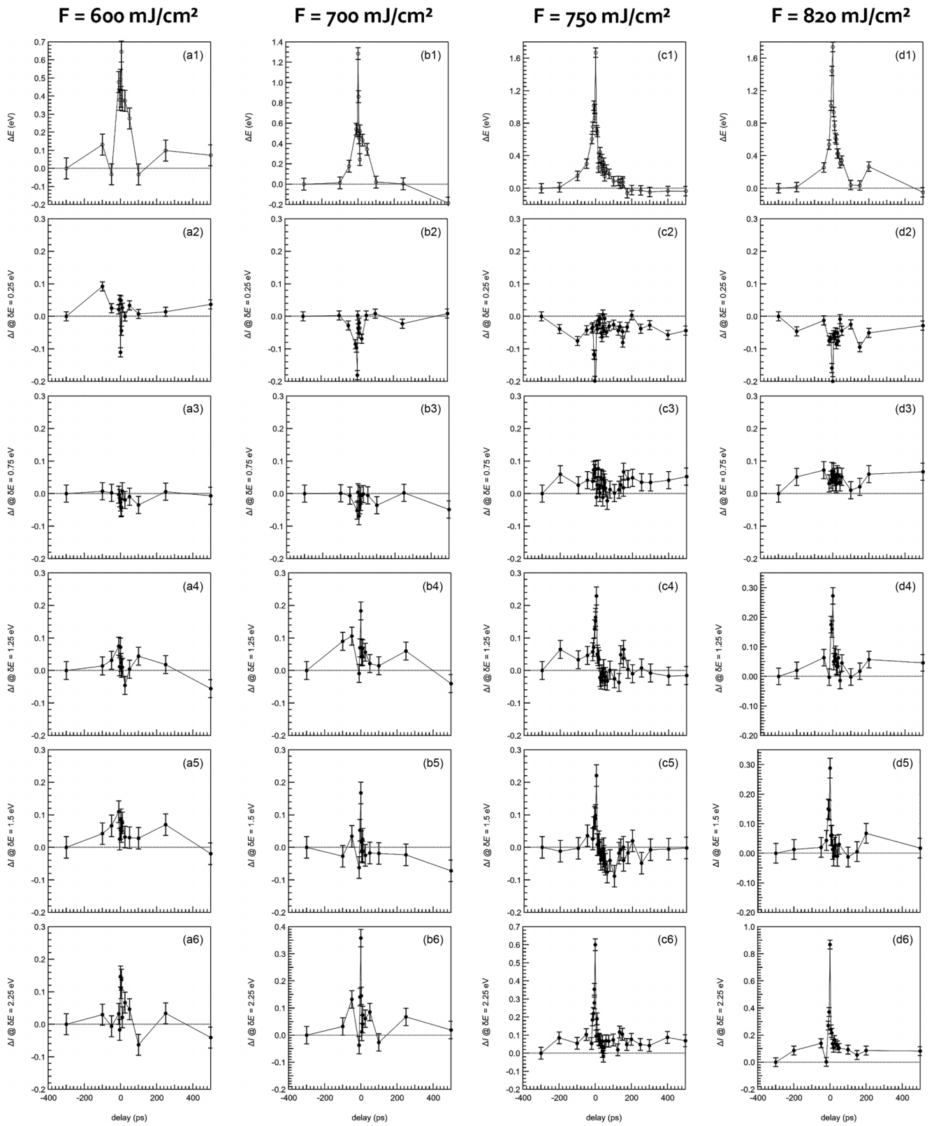
FIG. 10. Full set of experimental data for four different pump fluences: (a1)–(a6) F = 600 \text{ mJ/cm}^2 ; (b1)–(b6) F = 700 \text{ mJ/cm}^2 ; (c1)–(c6) F = 750 \text{ mJ/cm}^2 ; (d1)–(d6) F = 820 \text{ mJ/cm}^2 . Each row labeled from 1 to 6 respectively corresponds to (1) \Delta E spectral shift, (2) \Delta I(0.25 \text{ eV}) , (3) \Delta I(0.75 \text{ eV}) , (4) \Delta I(1.25 \text{ eV}) , (5) \Delta I(1.5 \text{ eV}) , and (6) \Delta I(2.25 \text{ eV}) .
