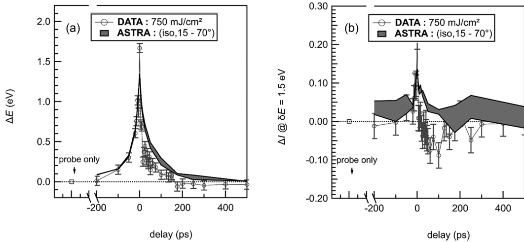
FIG. 16. Final experimental and ASTRA results comparison of the spectral shift \Delta E (a) and \Delta I(1.5 \text{ eV}) (b) for a fixed pump angular isotropic distribution and a Gaussian probe angular emission of 15 to 70° FWHM and JV1 configuration of the jellium-Volkov model.
