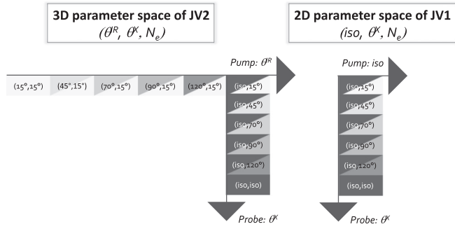
FIG. 11. Parameter spaces explored with the ASTRA space charge calculations for JV1 and JV2 configurations of the jellium-Volkov model. For each couple of pump/probe angular distributions (\theta_{\text{FWHM}/\text{iso}}^{\text{IR}}, \theta_{\text{FWHM}/\text{iso}}^{\text{X}}) , the number of pump electrons is varied in the range of about one order of magnitude in order to find the best agreement with the experimental results.
