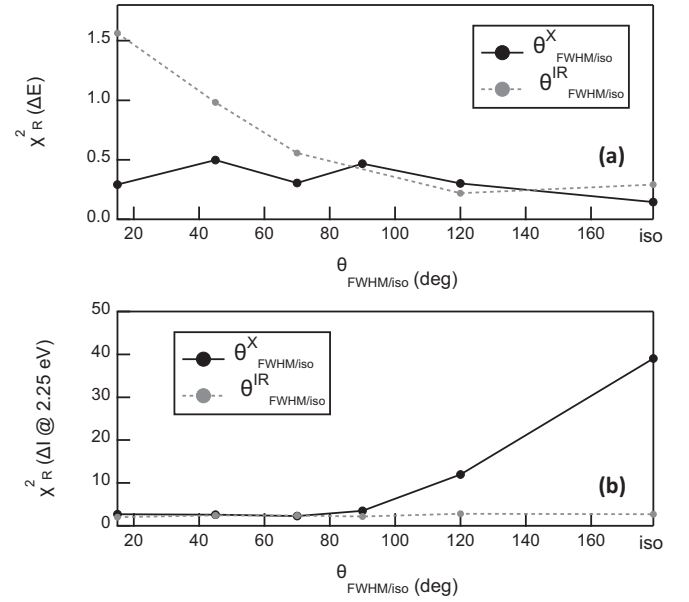
FIG. 13. Illustration of the pump and probe angular distribution optimization procedure. (a) Evolution of \chi_R^2 on the spectral shift in negative delays as a function of pump and probe \theta_{\text{FWHM}} . (b) Evolution of \chi_R^2 on the valence band shape modification \Delta I(2.25 \text{ eV}) as a function of pump and probe \theta_{\text{FWHM}} .
