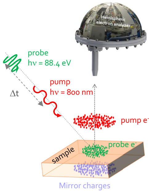
FIG. 4. Schematic representation of the pump/probe electron clouds emission.
