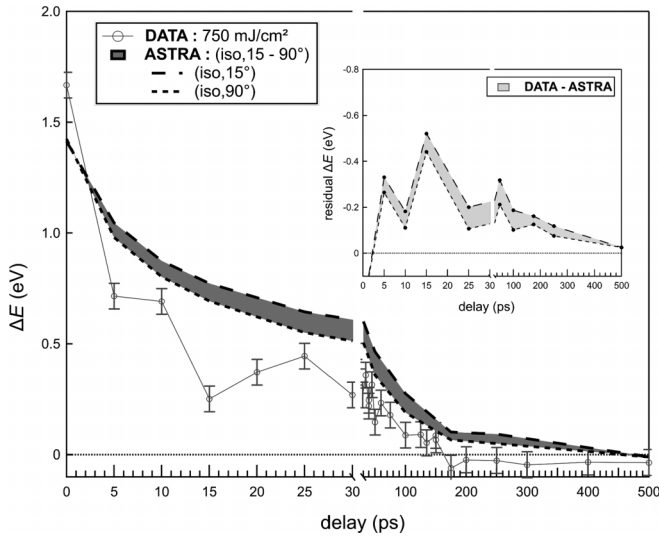
FIG. 6. Measured ( F = 750 \text{ mJ/cm}^2 ) and calculated (ASTRA; iso, 15\text{--}90^\circ ) shift \Delta E . Inset: residual shift after subtraction of the ASTRA shift to the measured one. The x axis is split in order to enhance the visibility of the short time dynamics.
