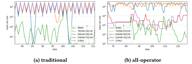
Figure 10: Evolution of input set sizes in their order of execution in online pipelines (log scale)
