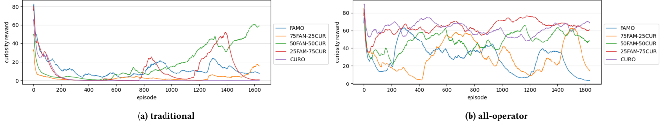
Figure 6: Evolution of intrinsic reward (curiosity-based) during training
