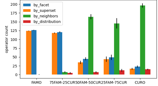
Figure 9: Operator distribution in online pipelines.
