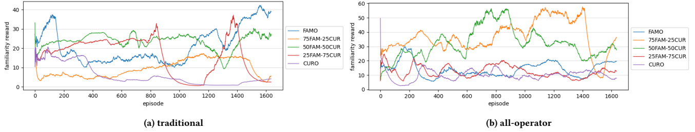
Figure 5: Evolution of extrinsic reward (familiarity-based) during training
