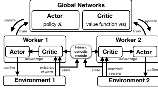
Figure 3: Architecture Details of Offline Training
