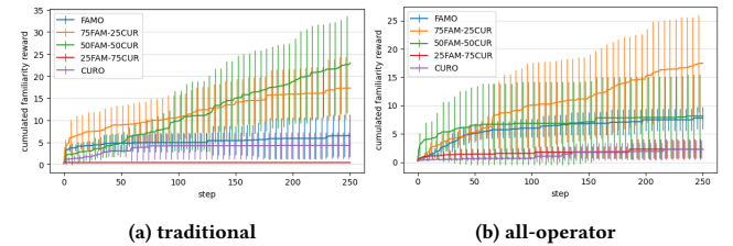
Figure 11: Evolution of the cumulative extrinsic reward during online pipelines
