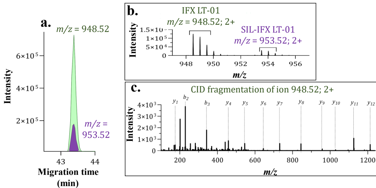
Fig. 6. Infiximab (IFX) and SIL-IFX peptide LT-01 (a) extracted ion electropherogram, (b) MS spectra ions, (c) MS/MS spectra of LT-01 ion.
