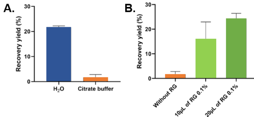
Fig. 5. Infliximab filtration recovery yield obtained using (A) H 2 O or citrate buffer solutions and (B) citrate buffer containing different quantities of surfactant (SF Rapigest). Experiments were performed in triplicates.
