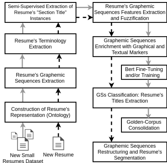
Fig. 4: A workflow derived by applying the proposed approach. Dotted black arrows illustrate how new resumes samples are processed based on a fine-tuned BERT-based model for extracting resume’s titles. Solid gray arrows indicate how new small resumes’ datasets can be exploited to fine-tune the BERT classifier
