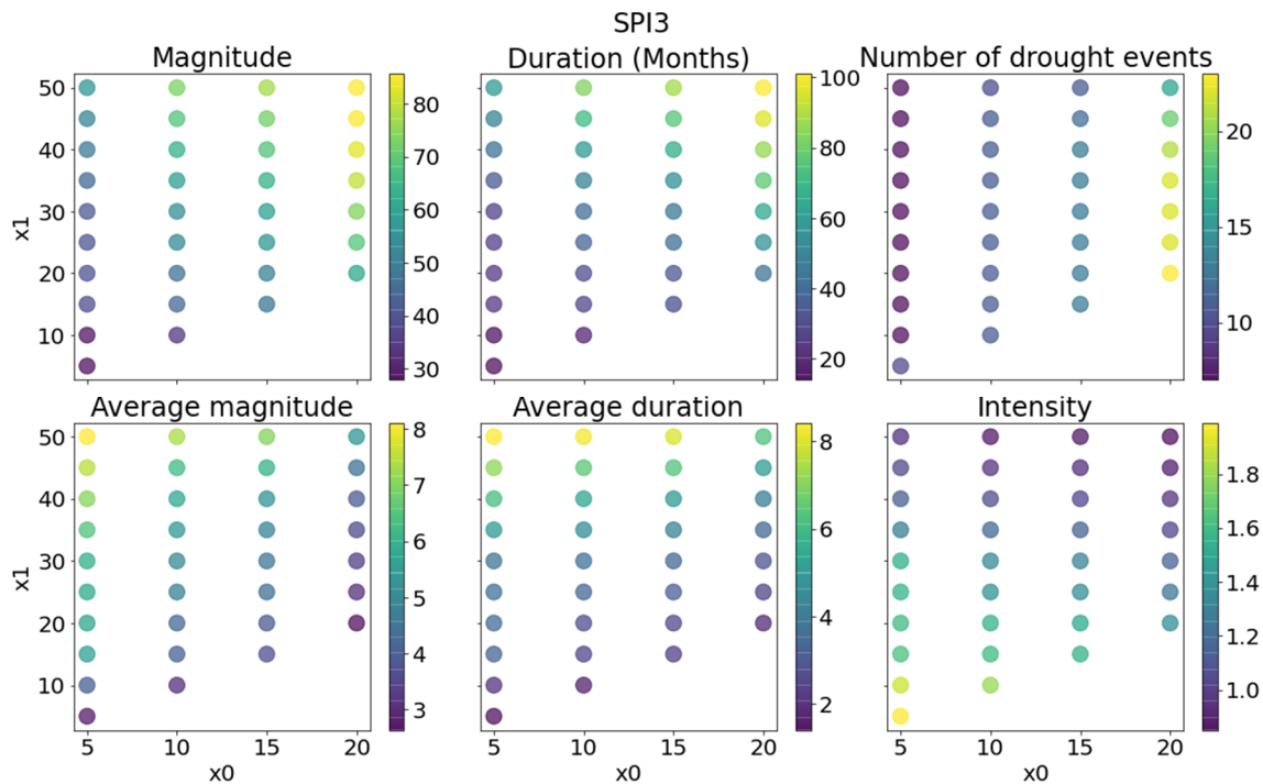
Figure 9. Drought characteristics and their averages extracted from SPI3 time series for several thresholds over the last 20 years (2001–2021).
