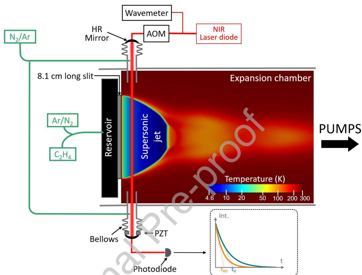
Fig. 1. Experimental setup used to record ethylene spectra (AOM: Acousto-optic modulator; PZT: piezoelectric transducer; HR Mirror: high-reflectivity mirror).
