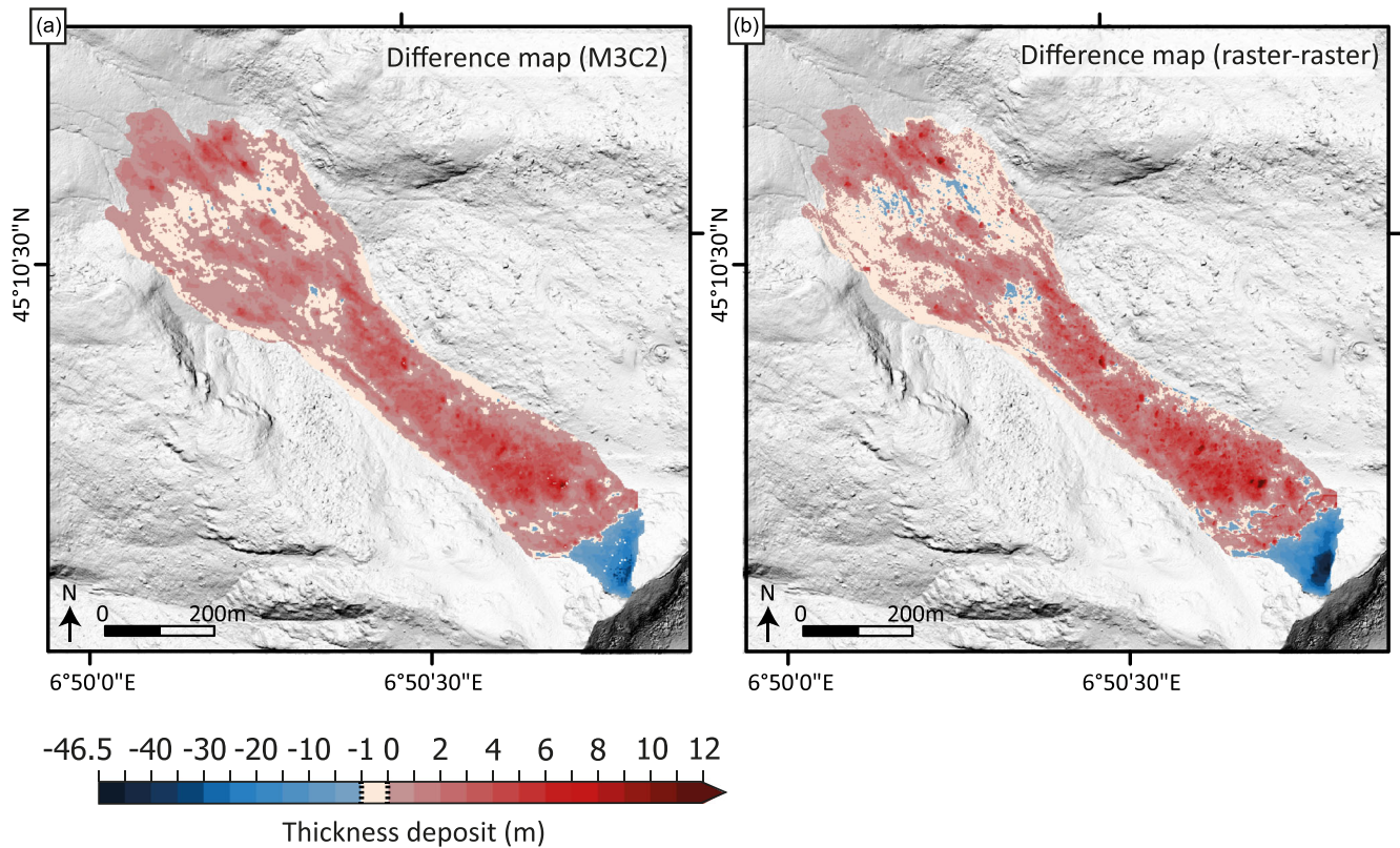
FIGURE A2 Difference maps of the deposition area obtained with two different methods of calculation (2D and 3D point cloud difference). [Color figure can be viewed at wileyonlinelibrary.com ]
