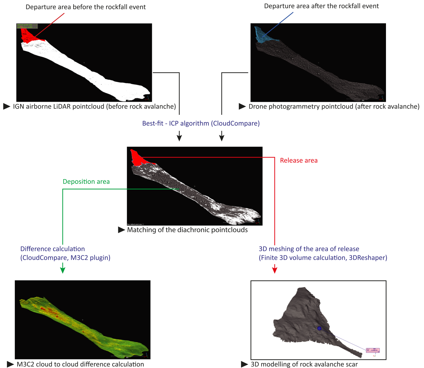
FIGURE A1 Methodology, data and the different steps that were used to perform volume calculations on the Étache rock avalanche event. [Color figure can be viewed at wileyonlinelibrary.com ]
