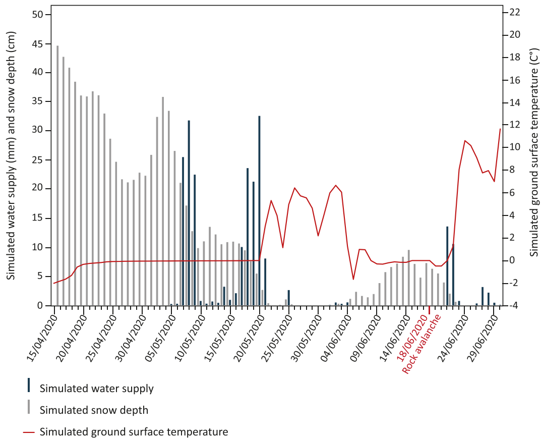
FIGURE 12 Simulated water supply (snowmelt and rainfall), snow depth and ground surface temperature at the scar altitude (elevation 3,108 m; aspect 320°, slope 32°). [Color figure can be viewed at wileyonlinelibrary.com ]
