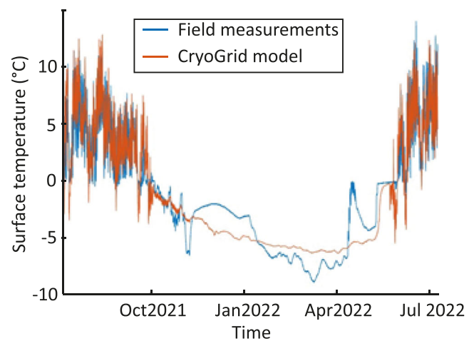
FIGURE B1 Comparison of measured and simulated surface temperature for sensor ETA_4 using the best fitting model parameters. [Color figure can be viewed at wileyonlinelibrary.com ]
