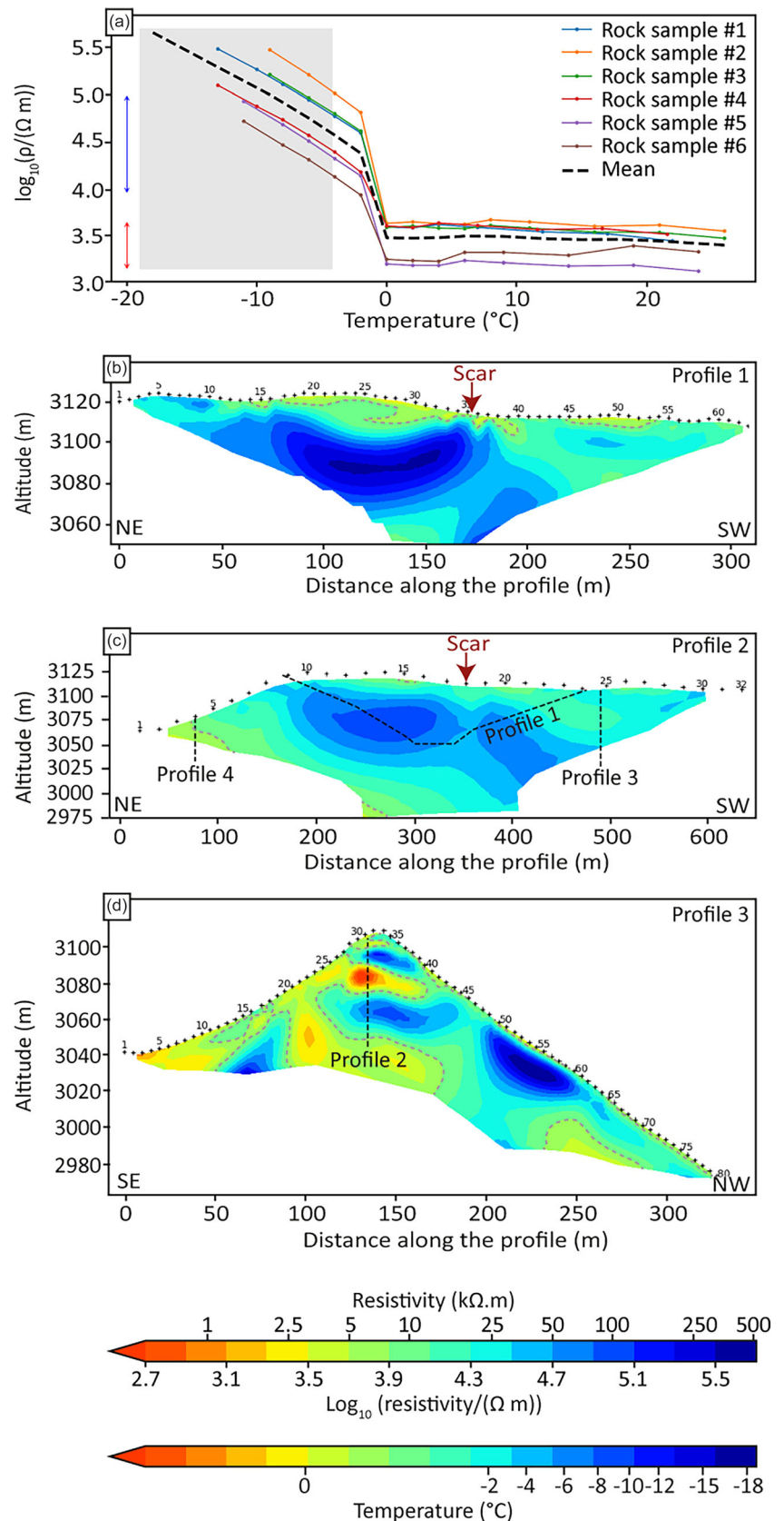
FIGURE 14 ERT profiles. (a) Resistivity as a function of temperature for the six rock samples. Arrows show the range of resistivity values from laboratory measurements for unfrozen rock (red arrow) and frozen rock (blue arrow, for temperature down to -4^{\circ}\text{C} ); the grey shading outlines the laboratory measurements below -4^{\circ}\text{C} , which is very unlikely to occur in the field according to the results of the heat transfer model. (b) Profile 1. (c) Profile 2. (d) Profile 3. Location of profiles is shown in Figure 9a. In figure (b), (c) and (d) the dotted grey line denotes the limit between the frozen and unfrozen areas, from laboratory measurements. [Color figure can be viewed at wileyonlinelibrary.com ]
