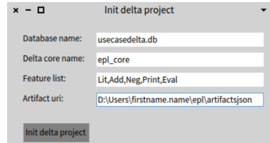
Figure 9: Graphical User Interface (GUI) displaying an example of User-Provided Data for initializing the Delta Project in PhaDOP.
