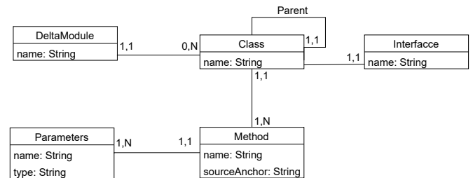
Figure 8: Metamodel structuring the repository for capturing reusable artifacts related to method implementation.
