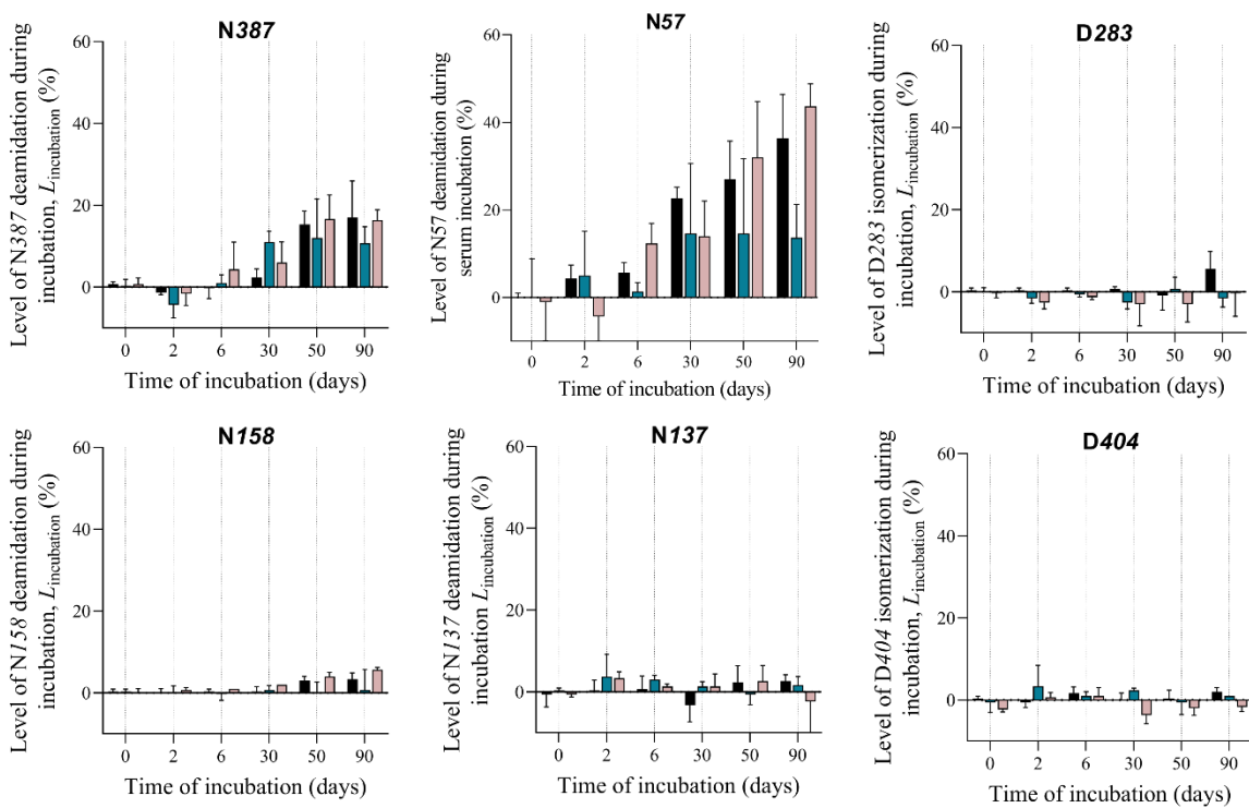
Fig. 4. Modification levels of 6 amino acids generated after incubation of infliximab in serum at 37 °C. Black bars: Remicade®, blue bars: Inflectra® and pink bars: Remsima®. Error bars correspond to standard deviation of triplicates.
