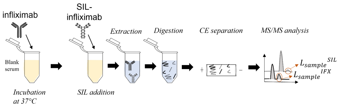
Fig. 2. Schematic representation of the CE-MS/MS strategy used to identify post-translational modifications (PTMs) of infliximab after incubation at 37 °C in serum.
