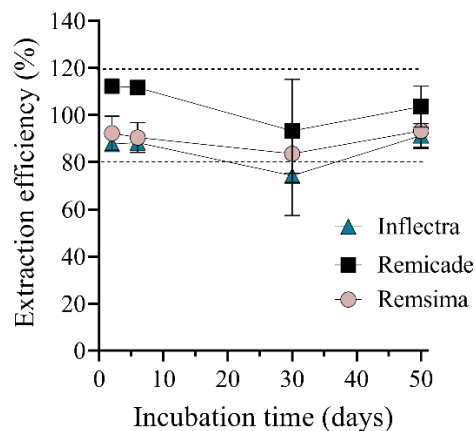
Fig. 5. Achieved extraction efficiency of infliximab innovator product (Remicade®) or biosimilars (Inflectra® and Remsima®) for different incubation duration in blank serums at 37 °C. Error bars represent the standard deviation among triplicates. Dotted lines: bias of +/- 20% of the extraction efficiency compared to a sample without incubation (reference).
