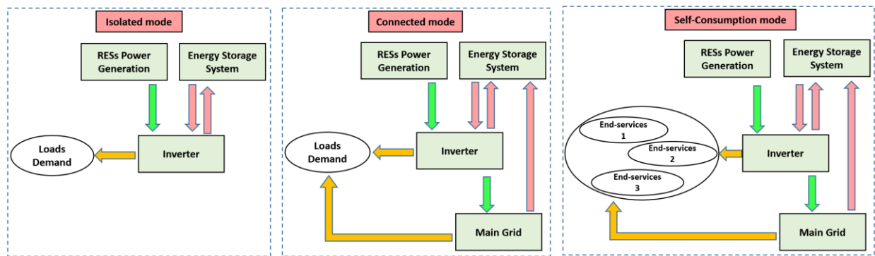
Figure 4. The MG system operating modes
