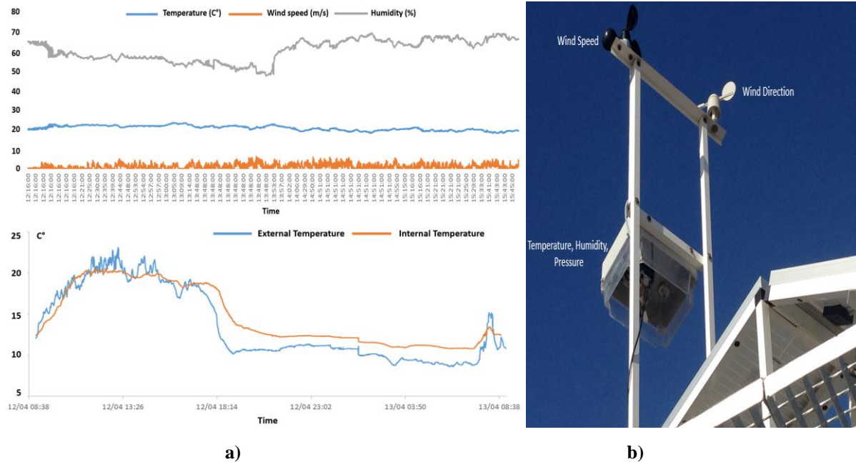
Figure 10. a) Internal/external temperature b) weather monitoring
