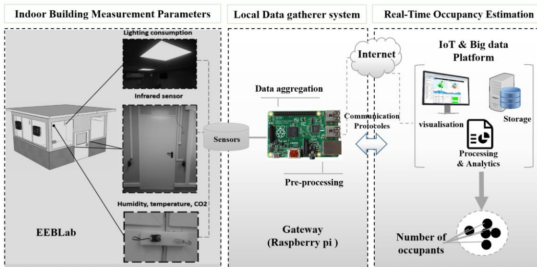
Figure 9. The architecture for occupants' presence detection/prediction and experimental results
