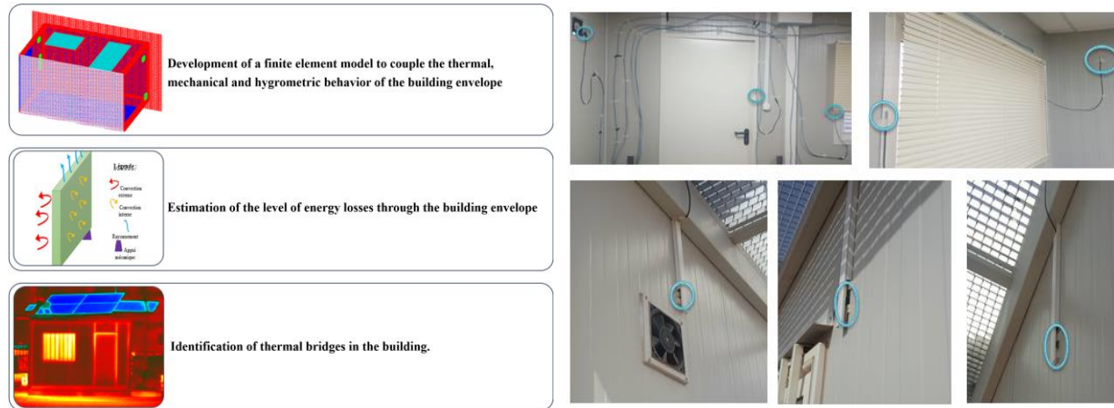
Figure 11. Thermal treatment of the front wall and the temperature sensors positioning [50]
