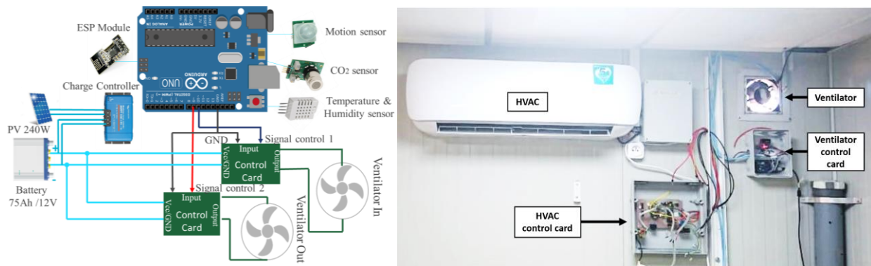
Figure 12. Context driven control card and active equipment control
