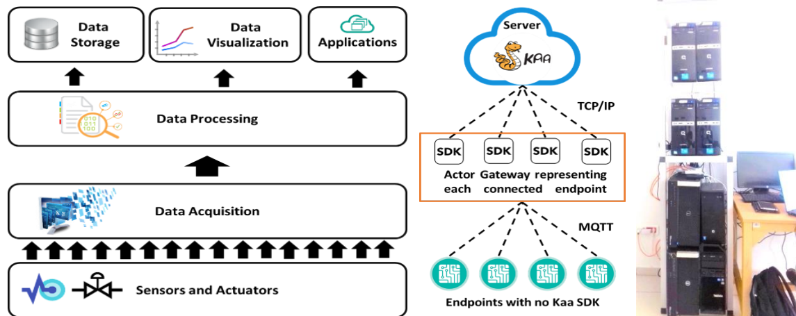
Figure 8. IoT/Big-Data platform architecture
