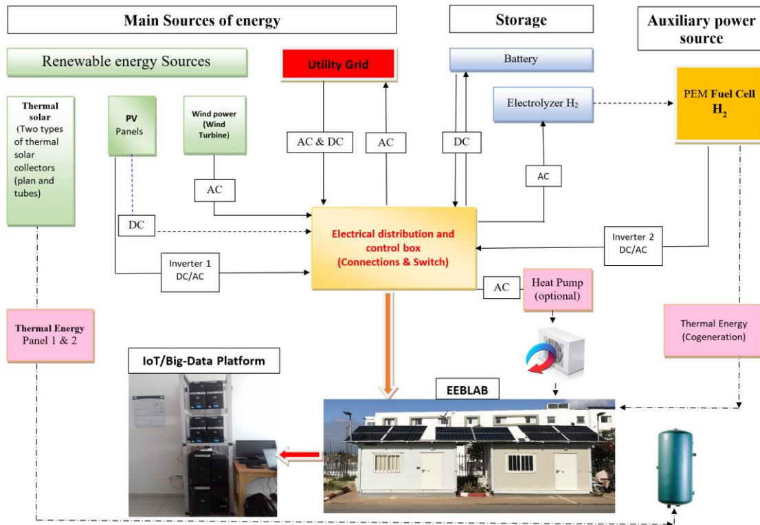
Figure 7. The holistic model of the deployed MG system
