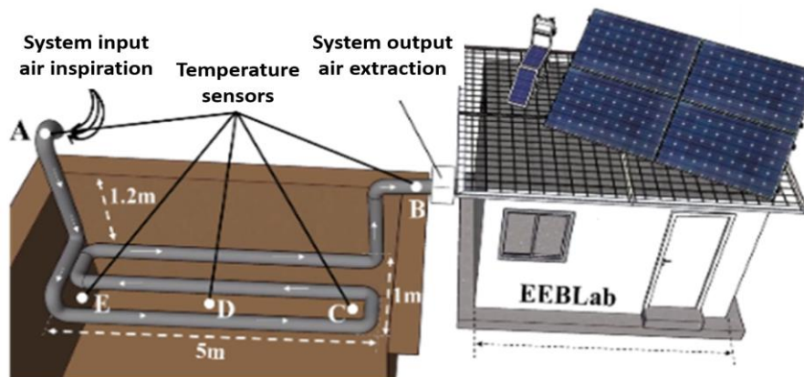
Figure 13. Geothermal installation in the EEBLab
