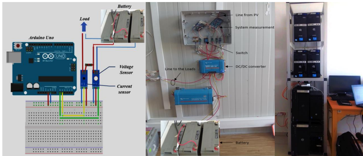
Figure 15. Battery characterization system
