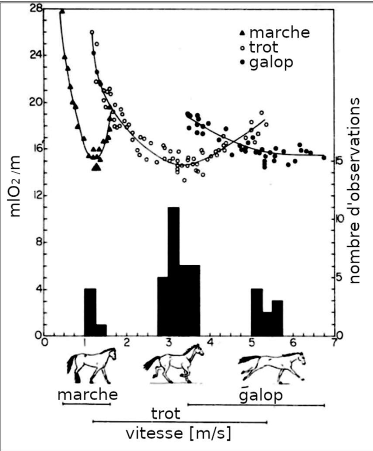
Cost of transport in horses D. F. Hoyt et C. R. Taylor, Nature, 1981.
