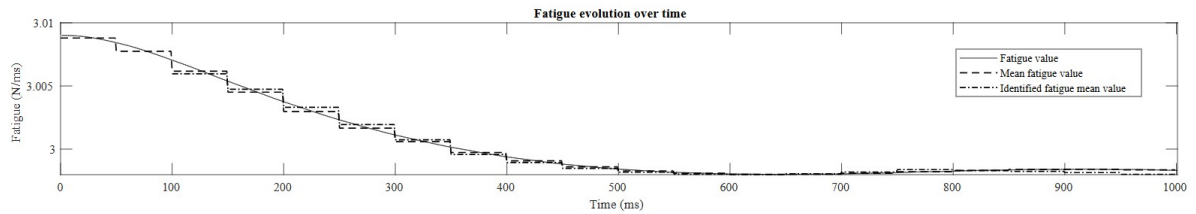
Fig. 4 Evolution of the fatigue (Ding model), mean fatigue values and identified mean fatigue values over time
