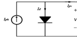
Figure 2. Equivalent circuit of a Shockley diode equation
