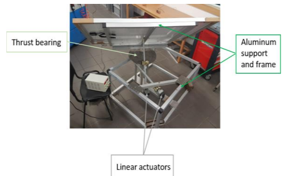
Figure 5. Mechanical prototype of the dual axis solar tracker
