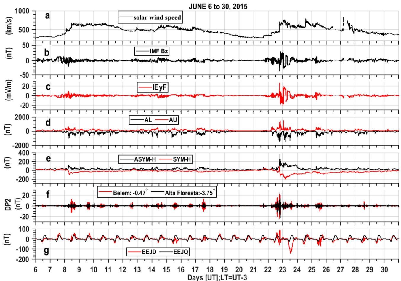
Figure 3. State of the interplanetary medium from 6 to 30 June 2015. (a) Velocity of the solar wind ( V_{sw} ). In addition, (b) shows the IMF B_z (interplanetary magnetic field in the Z direction), (c) presents the y-component of interplanetary electric field, (d) portrays the aurora electrojet (AL: aurora lower boundary, AU: aurora upper boundary), (e) demonstrates the H-component symmetry of Earth's magnetic field observed at various low latitudes, and (f) illustrates DP2 currents in Belem (dip lat: -0.47^\circ ) and Alta Floresta ( -3.75^\circ ). Further, (g) shows the day-to-day variations of EEJ current (red legend) and magnetically five-quiet day average (black legend).
