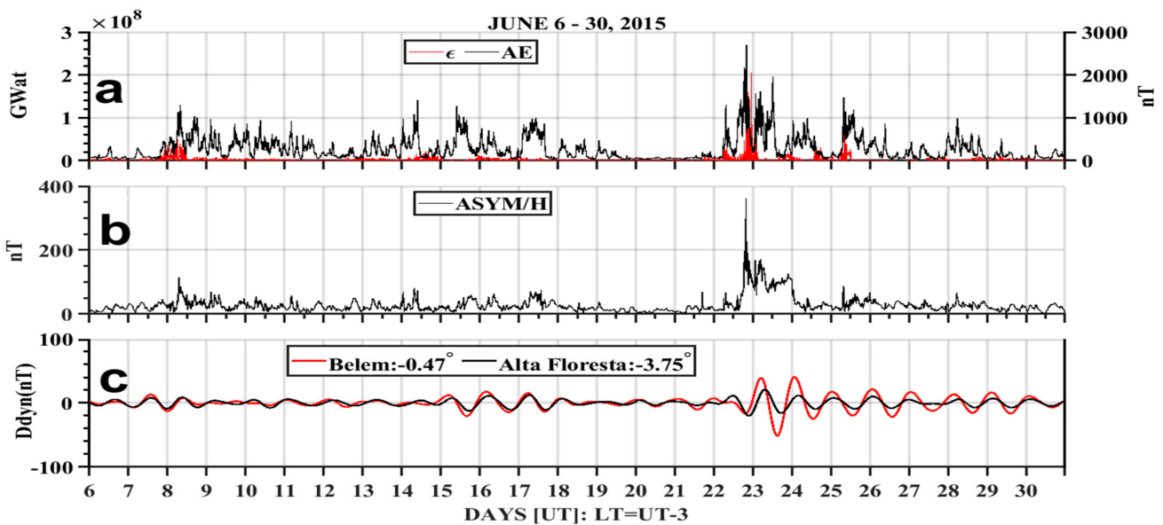
Figure 5. Variation in diurnal component of Ddyn alongside the AE index, Akasofu index, and ASYM-H index from 6 to 30 June 2015. (a) Day-to-day variation of the AE index (right-hand side of (a), presented in the black legend) and Akasofu index left-hand side of (a) presented in the red legend (b) ASYM-H index presented in (b). (c) Diurnal component of Ddyn at magnetic stations in Belem represented in the red legend and Alta Floresta represented in the black legend.
