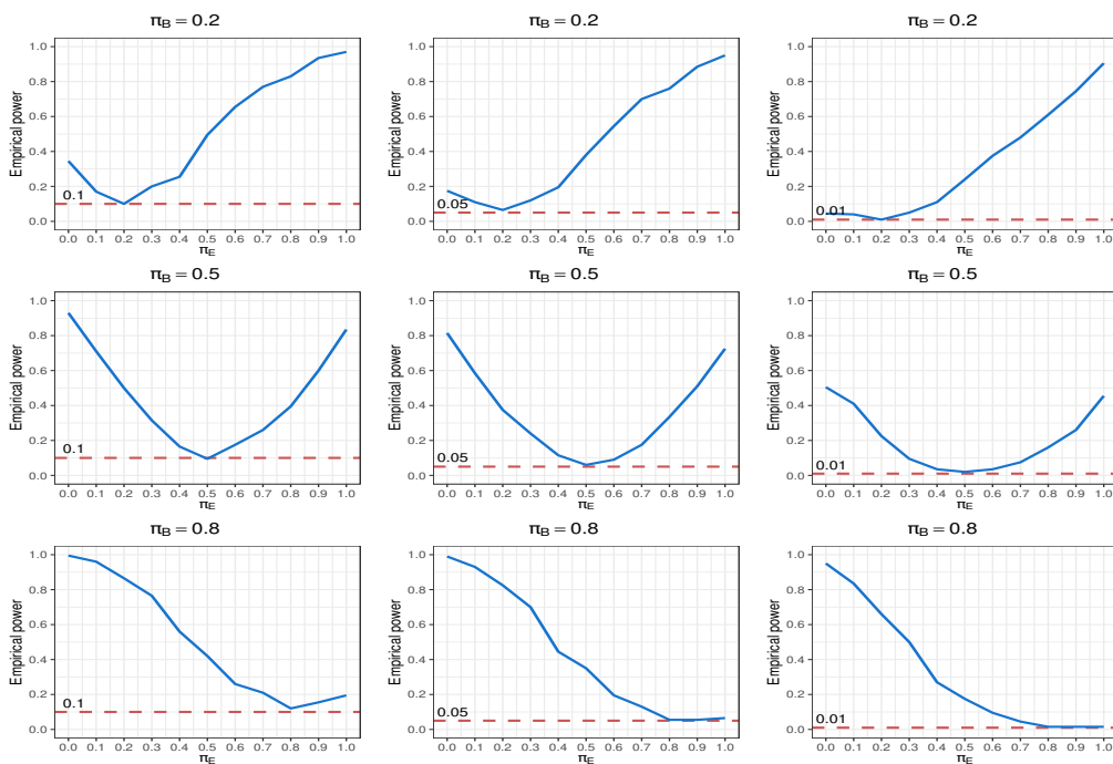
Figure 6: Empirical power of the test, based on 200 simulations of the model I with \phi_1 = 0.2 , \alpha_1 = 1 , \phi_2 = 0.7 , \pi_B is 0.2, 0.5 and 0.8 (for the top row, middle row, and bottom row respectively) and \pi_E \in \{0, 0.1, \dots, 1\} . The red horizontal dashed lines represent the significance level \alpha = 0.1, 0.05, 0.01 .
