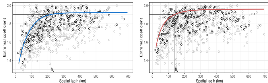
Figure 11: Extremal coefficient function for the first (1970-1990) and the last (2003-2023) windows in the left and right panels, respectively. Gray circles indicate the empirical pairwise estimates of the extremal coefficient; black ones are binned estimates (the number of bins equals 200). The blue and red curves show the theoretical extremal function of the model MM2 for the two considering time windows, respectively. The range of extremal dependence h_d is 213.94 km for the first window and 135.196 km for the last window.
