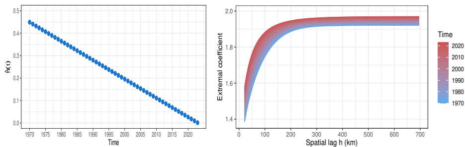
Figure 12: The left panel shows the temporal evaluation of the estimated mixing proportion \hat{\pi}(t) for the model MMM2 considering the time points from 1970 to 2023. The right panel displays the temporal evaluation of the extremal functions for the model MMM2. The blue curves represent the extremal functions for the most ancient time points, while the red curves represent those for the most recent ones.
