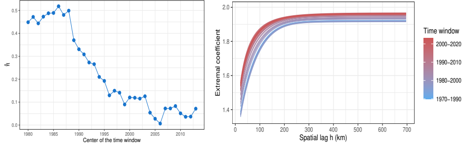
Figure 10: The left panel shows the temporal evaluation of the estimated mixing proportion \hat{\pi} for the model MM2 considering the 21-year time windows from (1970-1990) to (2003-2023), where its X-axis represents the center of the 21-year time window. The right panel displays the temporal evaluation of the extremal functions. The blue curves represent the extremal functions for the oldest time windows, while the red curves represent those for the most recent ones.
