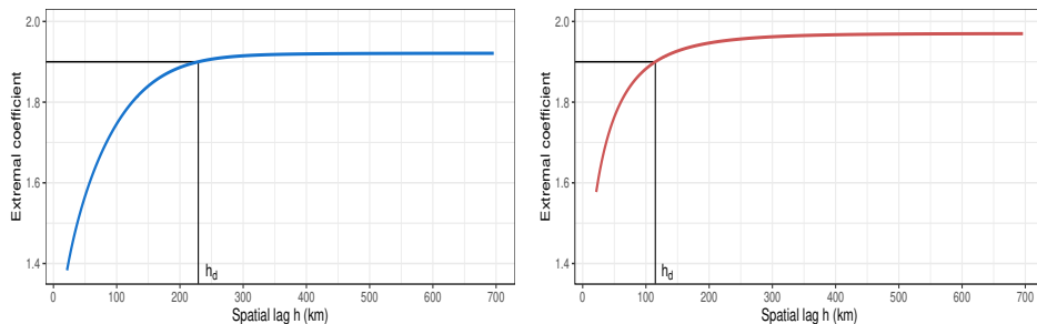
Figure 13: Theoretical extremal functions of the model MMM2 for the first time point (1970) and the last ones (2023) in the left and right panels, respectively. The range of extremal dependence h_d is 229.05 km for the first time point and 114.87 km for the last time point.
