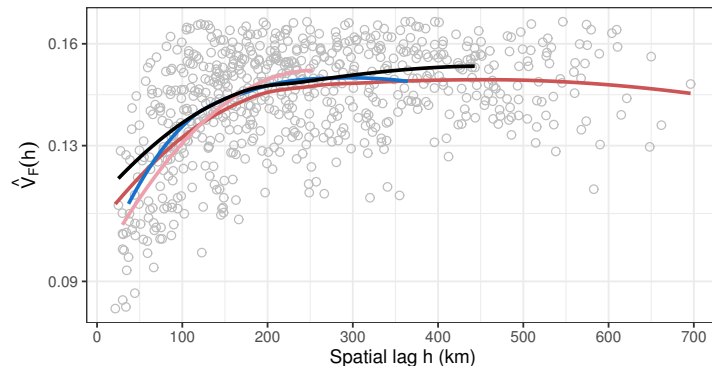
Figure 9: Empirical F-madogram of the yearly maxima (1970-2023). Gray circles represent the empirical values for all the pairs. The red, blue, pink, and black lines represent the smooth values of the empirical F-madogram using the pairs in the directional sector (-\pi/8, \pi/8] , (\pi/8, 3\pi/8] , (3\pi/8, 5\pi/8] and (5\pi/8, 7\pi/8] , respectively.
