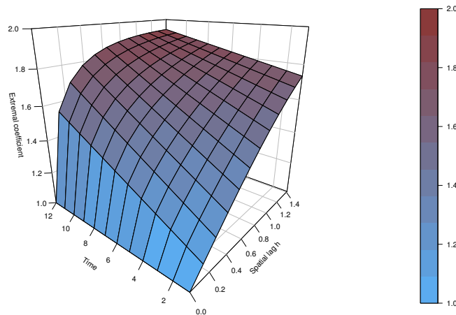
Figure 2: Surface plot for the extremal coefficient of the process which is shown in Figure 1.
