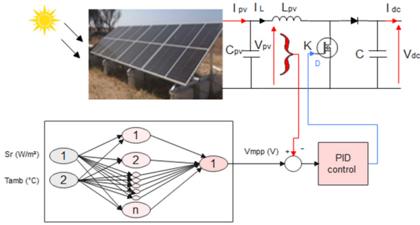
Fig. 4. The architecture of the ANN-based MPPT controller.
