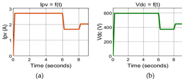
Fig. 7. PV-current (a) and DC-bus voltage (b) waveforms.
