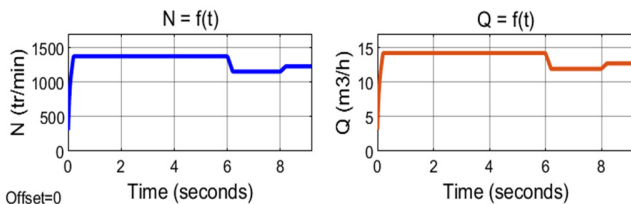
Fig. 8. The mechanical speed (a) and the flow rate (b) waveforms.
