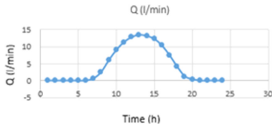
Fig. 14. Measurements of the water flow rate for one day in June 2023.
