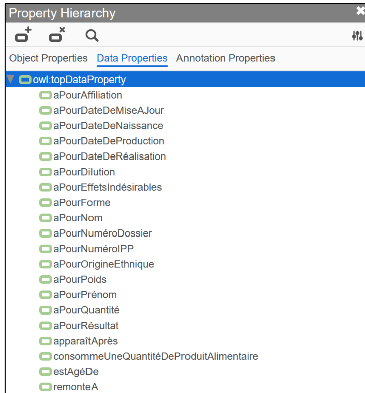
Fig. 8. Data properties represented in ALLERGIDOC ontology.
