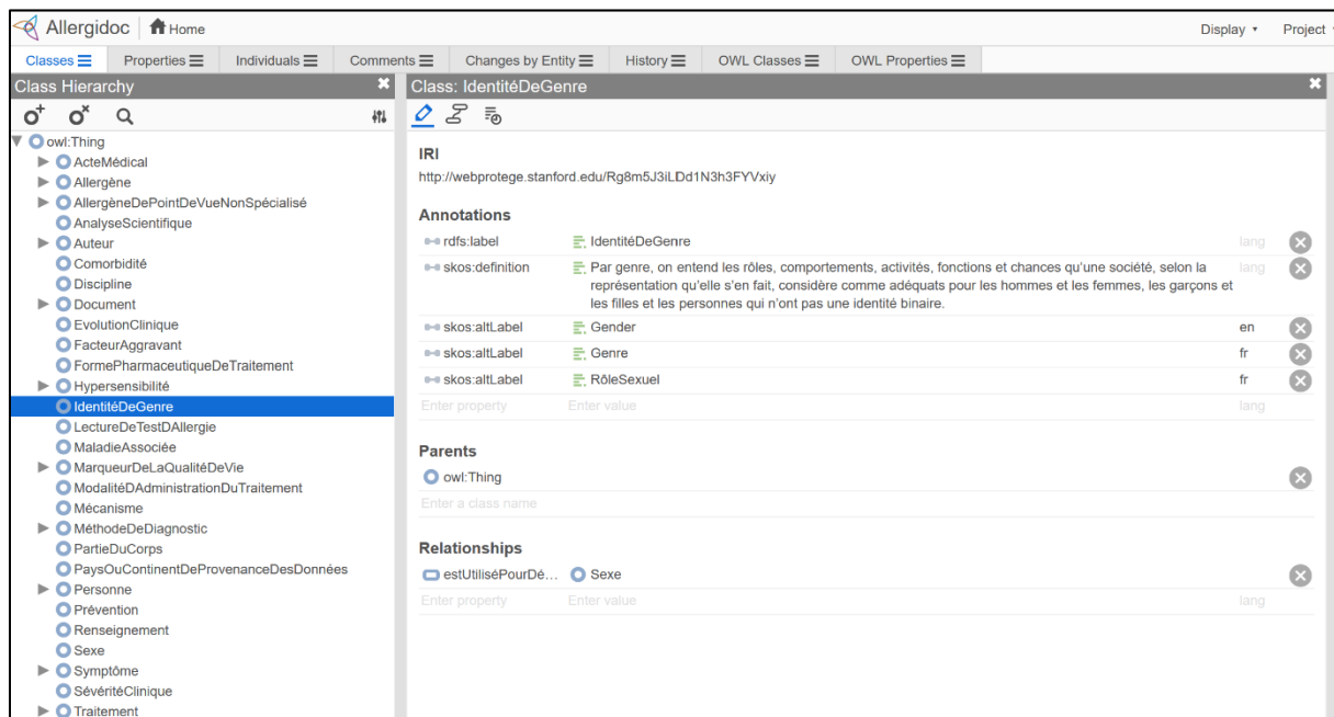
Fig. 5. Principal classes (facets) and its properties, represented in ALLERGIDOC ontology.
