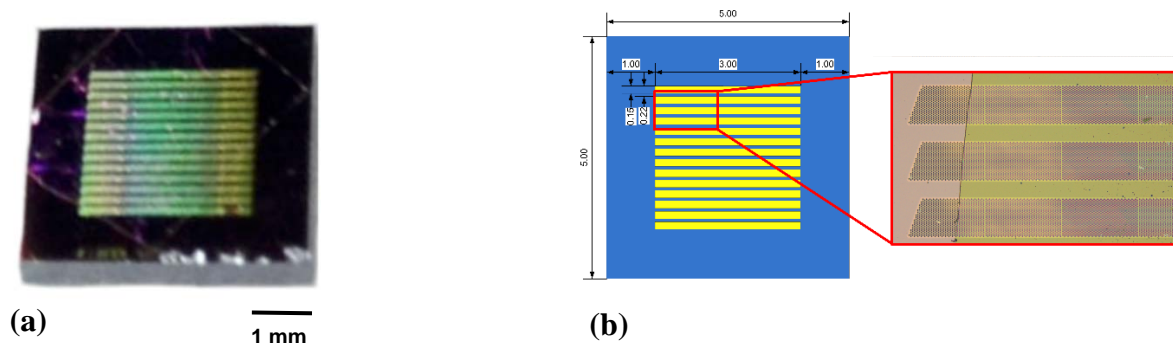
Figure 2. Details of the Si grid substrate (a) photo of Si grid and (b) design of Si substrate (left) and optical microscopy image of small region (right) showing 5 μm holes array with thin PS polymer film (area of greenish tinge); distances in mm.
