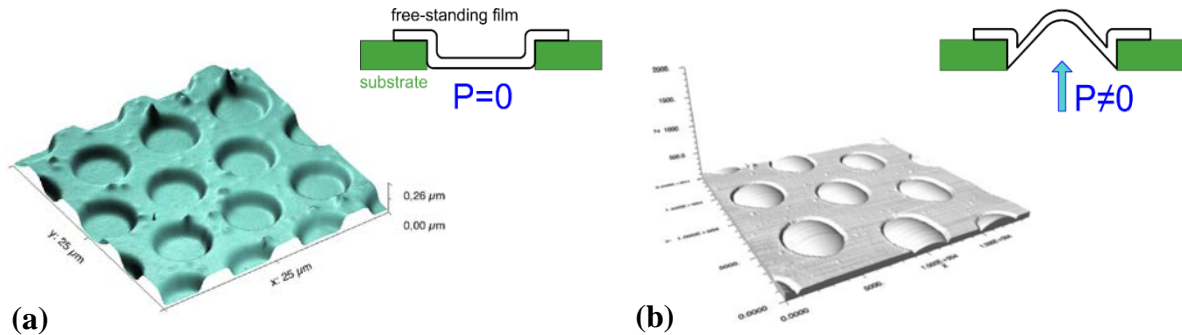
Figure 1. Examples of AFM measurements of films on 5 \mu\text{m} hole grid substrates (a) 90 nm thick PS film with T = \text{RT} and P = 0 Pa. Deflection due to capillary forces during the annealing process and (b) inflated 17 nm thick PS film with T = 57 ^{\circ}\text{C} and P = 1 psi ( \approx 69 kPa) [17].
