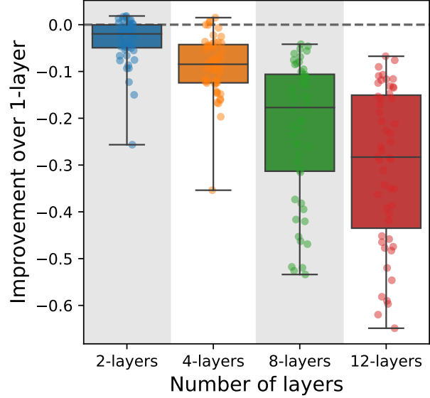
Figure 11. The effect of oversmoothing: comparing prediction from representations extracted from the GNN from the 2 nd , 4 th , 8 th , and 12 th layers, with that build from the first layer. We see that the deeper we go in the GNN, the less useful the representation is for downstream task. We interpret this as an effect of oversmoothing.
