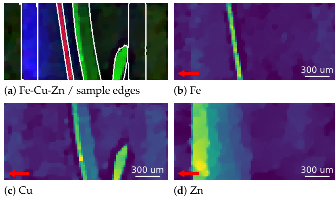
Fig. 5. (a) Composite image of Fe, Cu, Zn (Red, Green, and Blue respectively), and super-imposed edges of the transmission image in Fig. 2b; and the qualitative elemental reconstructions of: (b) Fe; (c) Cu; and, (d) Zn. The images are affected by self-attenuation of the XRF photons. The XRF detector position is indicated with a red arrow.
