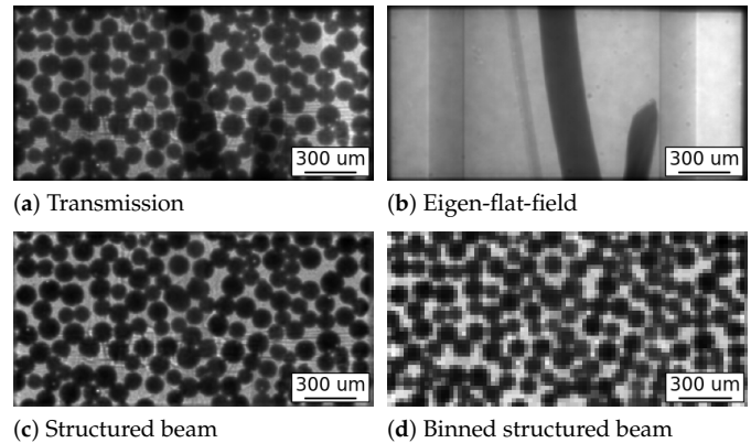
Fig. 2. (a) Transmission image of the sample with the mask; (b) eigen-flat-field computed from the stack of transmission images; (c) the extracted mask from transmission (normalized and mean-subtracted); and, (d) its 4 \times 4 binned version. The intensity gradient in (a) and (b) is due to the fact that the sample is not correctly positioned in the center of the beam. This effect is correctly taken into account by the eigen-flat-field subtraction when retrieving (c).
